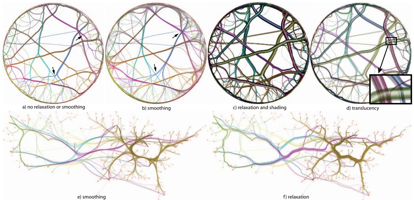
Fig. 6. Layout postprocessing. Edge smoothing (a vs b, Fig. 7 j vs e). Edge relaxation (Fig. 7 j vs f). Cushion shading (c), see-through detail (d).
