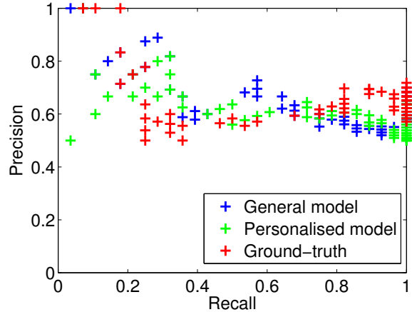
Figure 6: Precision and Recall values of abnormal event detection using our estimated and the ground-truth pose. Blue: estimated pose from our general model, green: estimated pose from our personalised model, and red: ground-truth pose.
