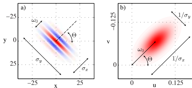
Figure 6: Gabor filter: a) spatial domain, b) frequency domain. Parameters: \sigma_x = 5 , \sigma_y = 10 , \omega_0 = 0.1 , \Theta = \pi/4
