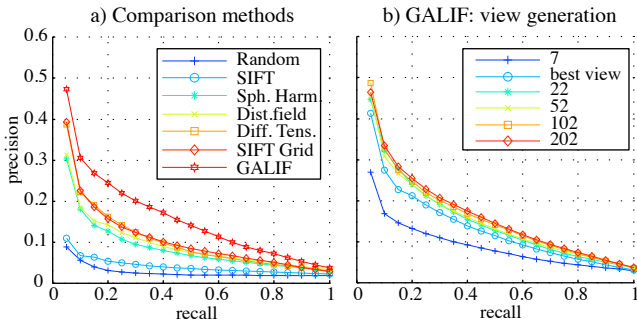
Figure 9: Detailed evaluation of retrieval performance on test dataset (higher curves are better): a) comparison with previous work using optimized system parameters; b) GALIF descriptor: influence of view generation methods.
