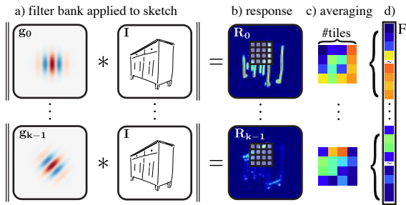
Figure 7: GALIF feature extraction pipeline: a) we convolve the input sketch \mathbf{I} with a filter bank of differently oriented Gabor filters \mathbf{g}_i to yield b) response images \mathbf{R}_i . The average responses c) within cells of a local patch form d) a local feature vector \mathbf{F} .
