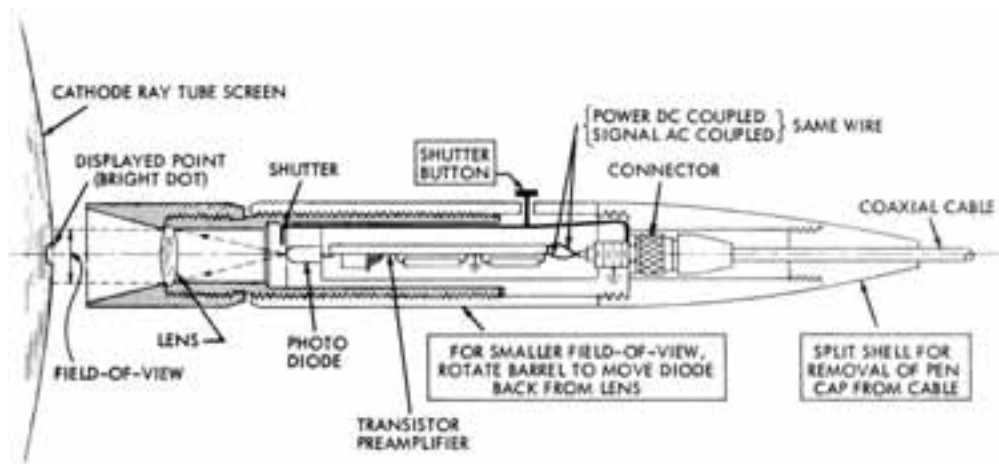
Figure 4.2: CONSTRUCTION OF LIGHT PEN. Drawing courtesy of Electronic Systems Laboratory. This drawing was made by conventional methods. (Originally on page 56.)
