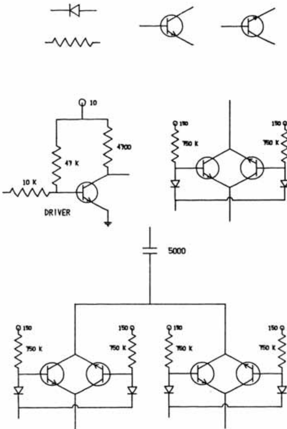
FIGURE 9.11. CIRCUIT DIAGRAMS
