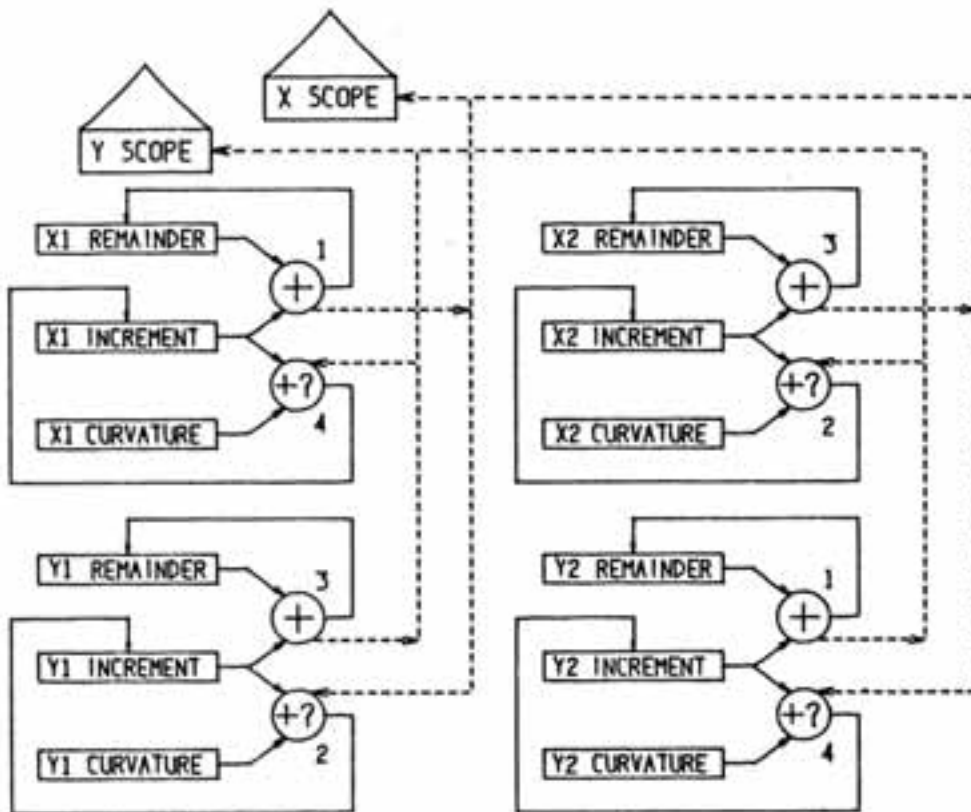
FIGURE E.3. DDA FOR THE GENERAL CONIC
