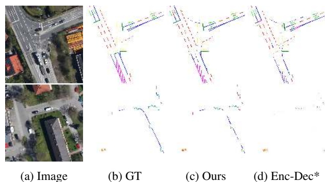
Figure 6: Result samples for the SkyScapes-Lane task by SkyScapesNet and the best baseline. Class colors: cf. fig. 2.
