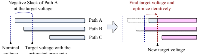
Fig. 4. Target voltage and path slack before and after slack optimization using the heuristic.
