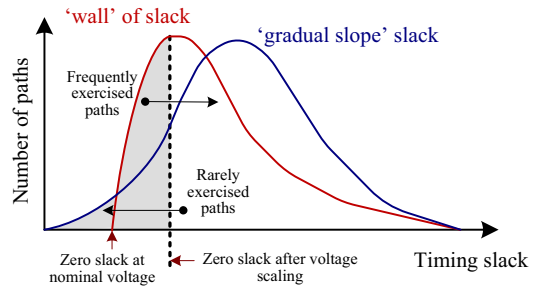
Fig. 2. The goal of the ‘gradual slope’ slack optimization is to transform a slack distribution having a critical ‘wall’ into one with a more gradual failure characteristic.
