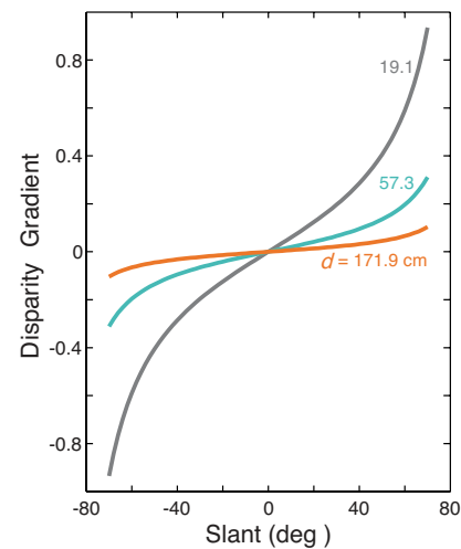
Figure 13. Disparity gradient as a function of slant at different viewing distances. The disparity gradient was calculated from Equation 12.
