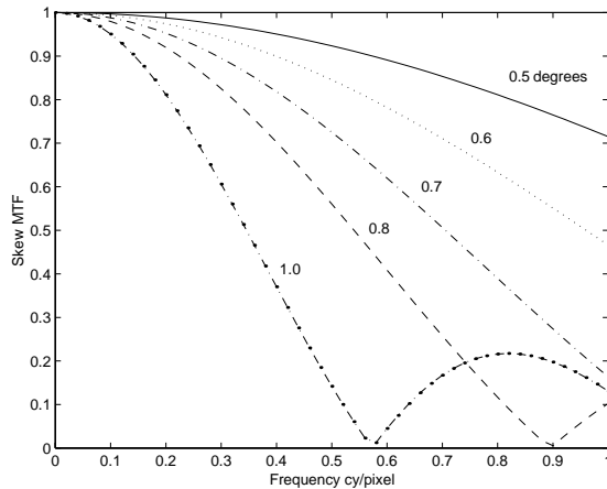
Figure 3. Skew MTF caused by various levels of angular error. The number of lines of data, m = 100 .
