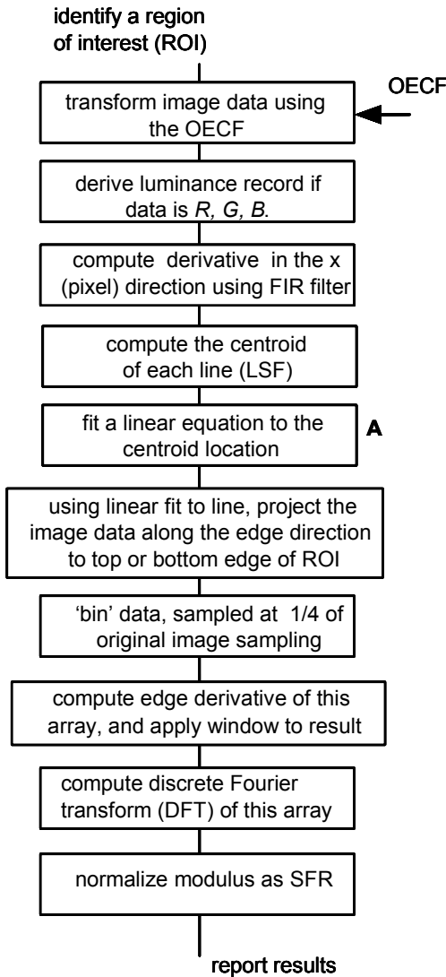
Figure 2. Description of the ISO 12233 spatial frequency response evaluation method. The edge is assumed to be oriented in a near-vertical direction. This figure has been edited to correct an error in the published PICS 2000 Proceedings.
