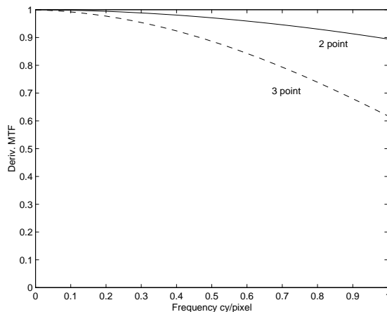
Figure 4. MTF caused by computation of the edge gradient by a finite difference. The 3-point difference [-0.5 \ 0 \ 0.5] is used in the ISO procedure.
