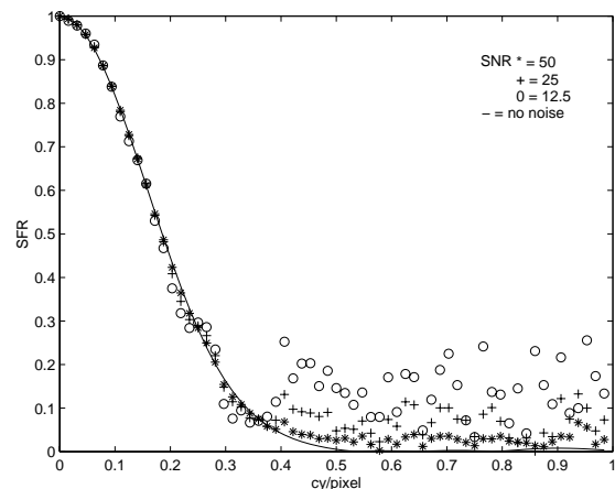
Figure 5. SFR based on 128 \times 64 data, for three levels of image noise. Noise is zero-mean, normally distributed and spatially uncorrelated
