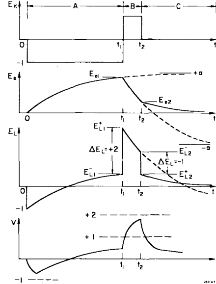
FIG. 3--Direct wave E_K , emitted wave E_e , and net load wave E_L for SLED.
