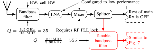
Fig. 9: Simplified block diagram for a narrowband WuRx, in red, partly reusing the main receiver's front end.
