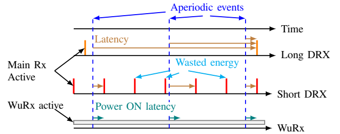
Fig. 6: DRX and wake-up receiver comparison.
