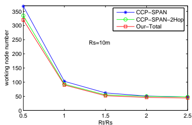
Fig. 13: Working node count vs. R_t/R_s ratio.
