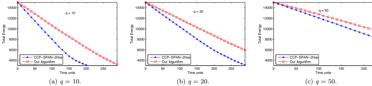
Fig. 19: Total energy in nodes in a sample run with different q values.
