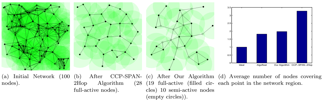
Fig. 15: Sample network snapshots before and after running two algorithms.
