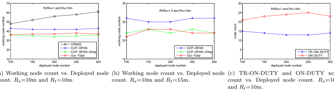
Fig. 12: Working node counts and their distribution in our protocol.
