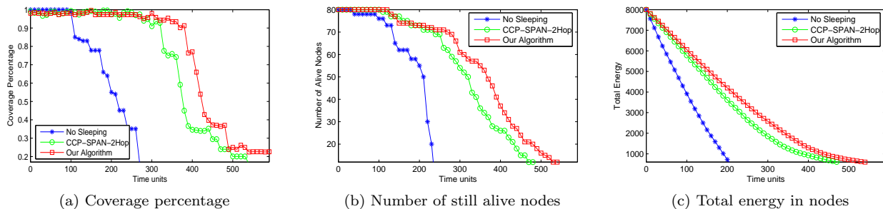
Fig. 18: Network statistics from a sample run when R_t/R_s = 1.5 .
