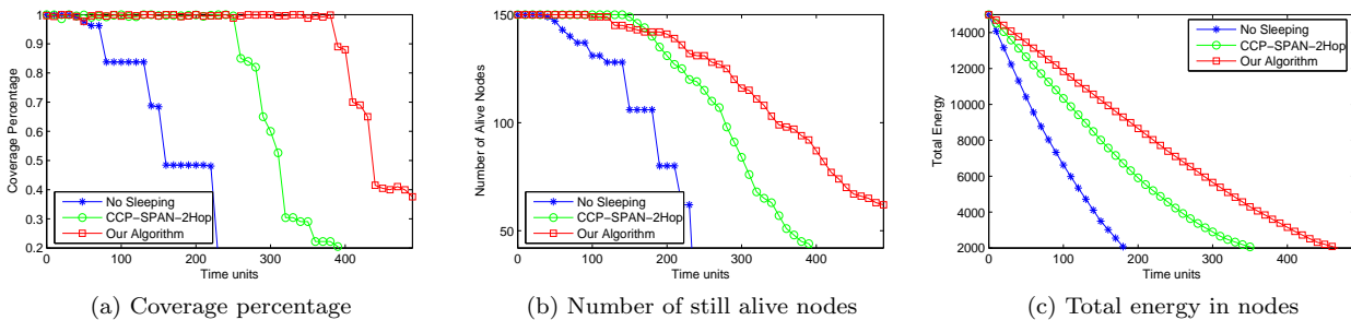
Fig. 17: Network statistics from a sample run when R_t/R_s = 1 .
