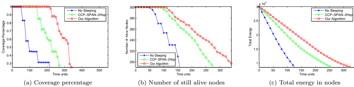
Fig. 16: Network statistics from a sample run when R_t/R_s = 0.5 .
