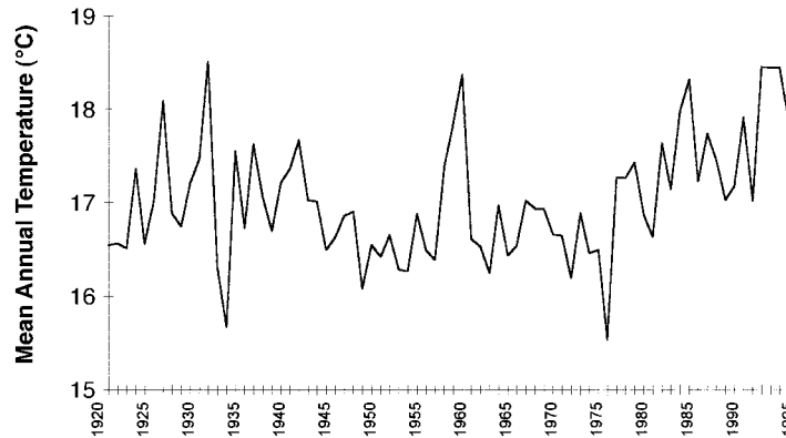
FIG. 2. Annual means of surface temperature from the Scripps Institution of Oceanography pier, 1920–1995. Although there is considerable interannual variability, average temperature has clearly been rising since the onset of the regime shift in about 1976 (McCall 1996).
