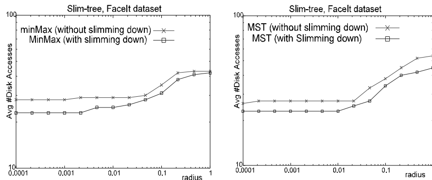
Fig. 6. Comparing the improvements given by the Slim-down algorithm to answer range queries.
