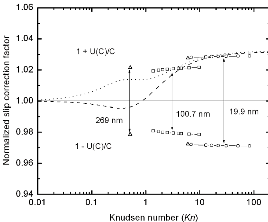
Fig. 13. Comparison of the slip correction factors for the reported PSL particle cases with our measurement result. The dashed line is for Allen and Raabe (1985), the dotted line is for Hutchins et al. (1995), and the solid line is for the current study. Confidence intervals for the expanded (2 sigma) uncertainty, U(C) , are given for our data.
