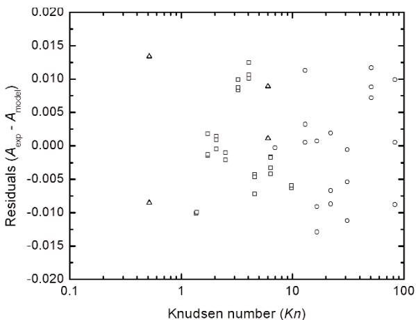
Fig. 9. Residuals for slip correction parameter measurements to the fitted model. Circle (19.90 nm), square (100.7 nm), and triangle (269 nm).
