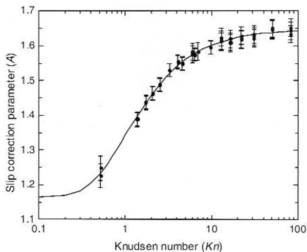
Fig. 11. Slip correction parameter A , measured and fitted. The bars represent the combined uncertainty.
