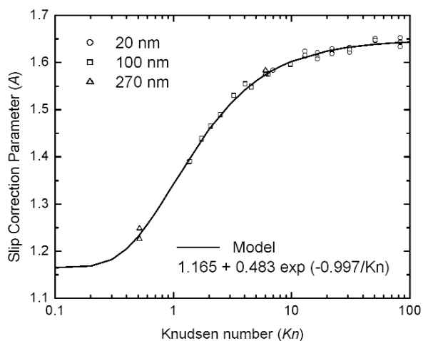
Fig. 8. Slip correction parameter A from the measurement of 20 nm, 100 nm, and 270 nm particles.
