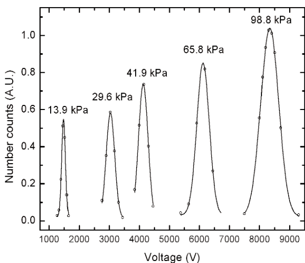
Fig. 4. Peak voltage shift at reduced pressure conditions for the 100 nm, SRM 1963 particles. The peak locations were adjusted to a sheath air flow condition of 100 \text{ cm}^3/\text{s} and the peak number concentrations were expressed in arbitrary units (A.U.) to fit on the graph.
