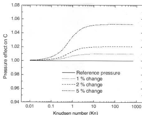
Fig. 6. Effect of pressure uncertainty on the measurement of the slip correction factor.
