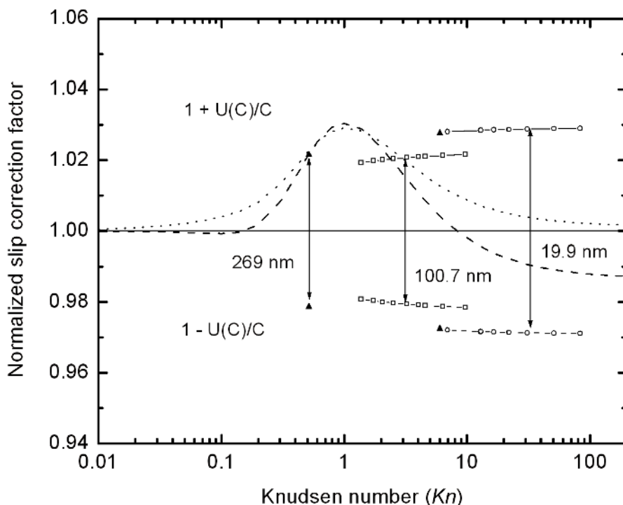
Fig. 14. Comparison of the slip correction factors for the reported oil drop cases with our measurement result. The dashed line is for Allen and Raabe (1982), the dotted line is for Rader (1990), and the solid line for the current study. Confidence intervals for the expanded (2 sigma) uncertainty, U(C) , are given for our data.
