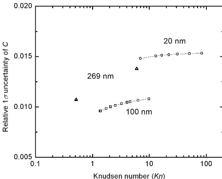
Fig. 12. Relative combined uncertainties of the slip correction factor C .
