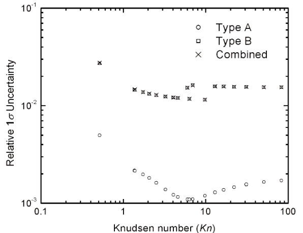
Fig. 10. Relative uncertainties of the slip correction parameter A .
