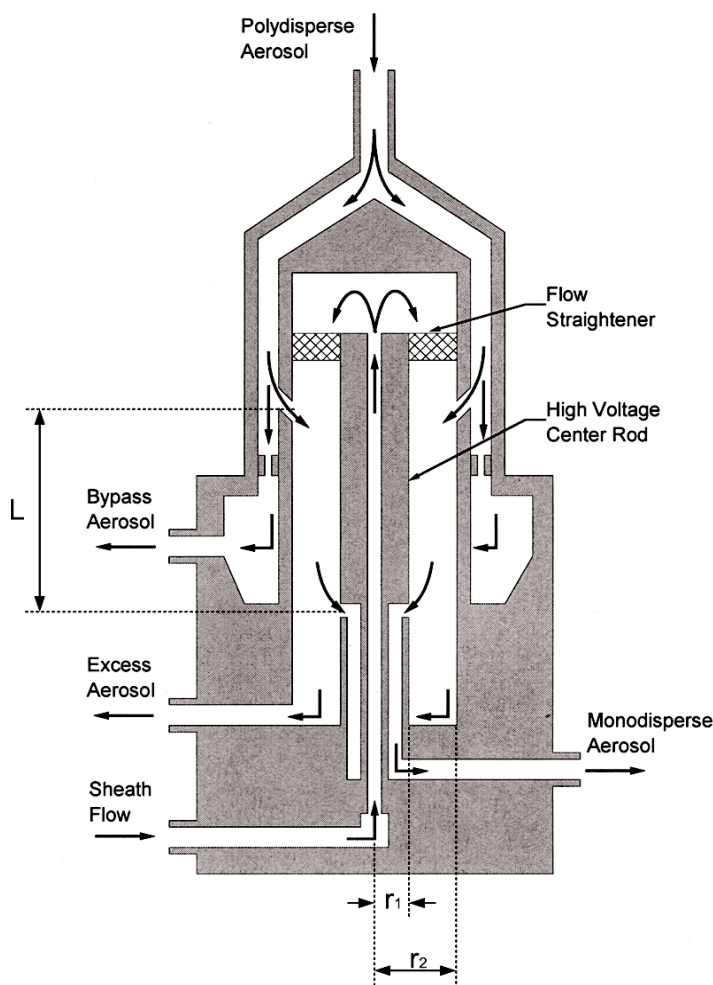
Fig. 2. Schematic diagram of an NDMA adapted from the TSI 3085 technical manual.
