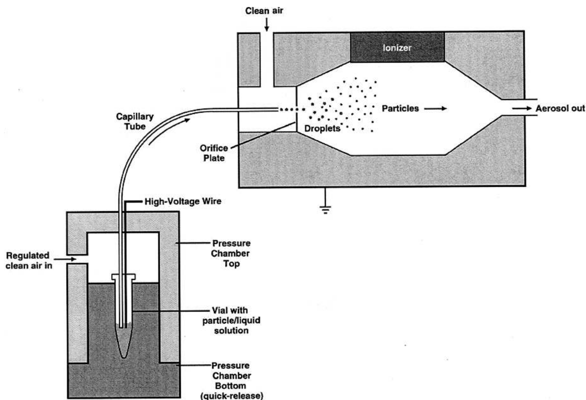
Fig. 1. Schematic diagram of the electrospay adapted from the TSI 3480 technical manual.
