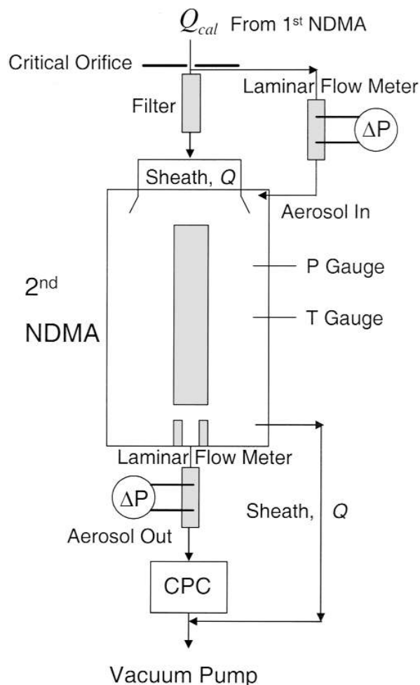
Fig. 3. Schematic diagram of the measurement NDMA system for reduced pressure conditions.
