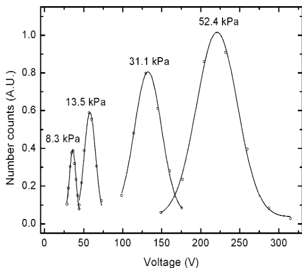
Fig. 5. Peak voltage shift at reduced pressure conditions for the 20 nm PSL particles calibrated using SRM 1963. The peak locations were adjusted to a sheath air flow condition of 100 \text{ cm}^3/\text{s} .
