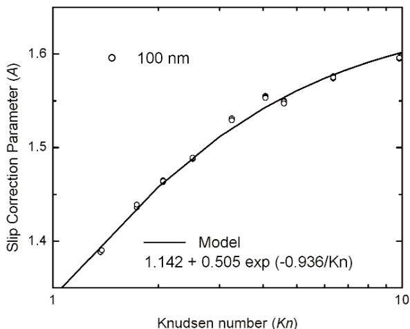
Fig. 7. Slip correction parameter A from the measurement of 100 nm particles, used in the size calculations for the 20 nm particles.
