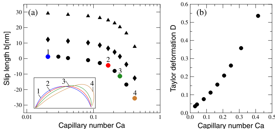
FIG. 3 (color online). (a) Slip length as a function of capillary number for a square array of bubbles with three different protrusion angles, \varphi = 63^\circ, 68^\circ, and 71^\circ (from uppermost to lowermost). In the inset cross sections of liquid-gas interfaces for four capillary numbers are shown. (b) Taylor deformation as a function of Capillary number for the bubble with \varphi = 71^\circ . These Ca values correspond to shear rates of the order of 10^{-6}-10^{-7} \text{ s}^{-1} .
