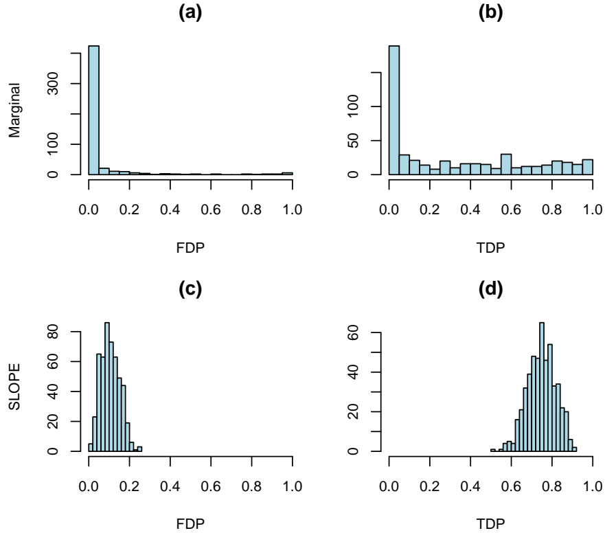
Figure 4: Testing example with q = 0.1 and k = 50 . Top row refers to marginal tests, and bottom row to SLOPE. Histograms of false discovery proportions are in the first column and of true discovery proportions in the second.
