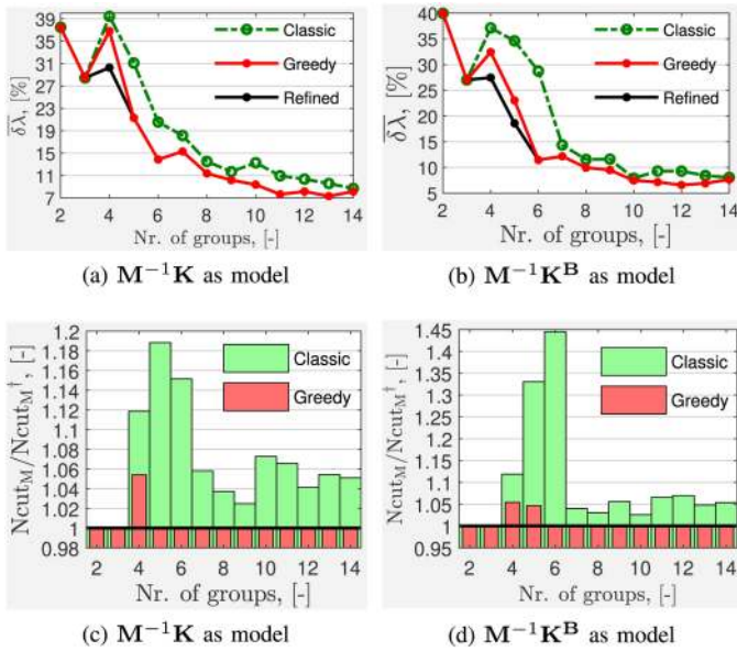
Fig. 3. Mean eigenvalue errors of inertial aggregate models based on groupings of the NPCC 48-machine system produced by three algorithms and associated generic Ncuts.
