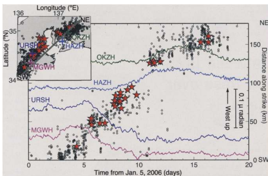
Fig. 3. Migration of seismicity of both VLF earthquakes and deep low-frequency tremors, and tilt change at four Hi-net stations—OKZH, HAZH, URSH, and MGWH—between 5 January and 25 January 2006. The temporal variation of VLF earthquakes (red stars) and deep low-frequency tremors (circles) is shown along the southwest-northeast line in the inset representing the strike of the subducting plate interface. The four colored lines are records of the east-west component of the tilt changes observed at Hi-net stations. The inset shows the distribution of the VLF earthquakes and deep low-frequency tremors during the same period, as well as the Hi-net TILT station locations (plus symbols).
