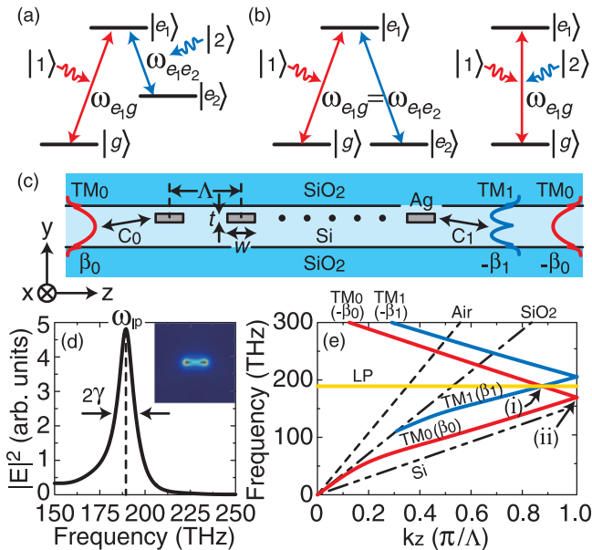
FIG. 1. (Color online) Schematics of (a) atomic EIT and (b) classical analogues. (c) Plasmonic resonator ( w/t = 50/5 nm) array embedded in a silicon waveguide with the core thickness of 600 nm. (d) |E|^2 spectral response of probe placed 5 nm from the resonator’s end facet and |E|^2 distribution of LP mode at resonance, \omega_{lp}/2\pi = 189 THz. (e) Numerically calculated dispersion relations of TM 0 and TM 1 bare modes for \Lambda = 275 nm. Coupled LP-TM 0 -TM 1 modes occur at the degeneracy point (i). When \Lambda is set at 240 nm, coupled LP-TM 0 -TM 0 modes occur at the point (ii).
