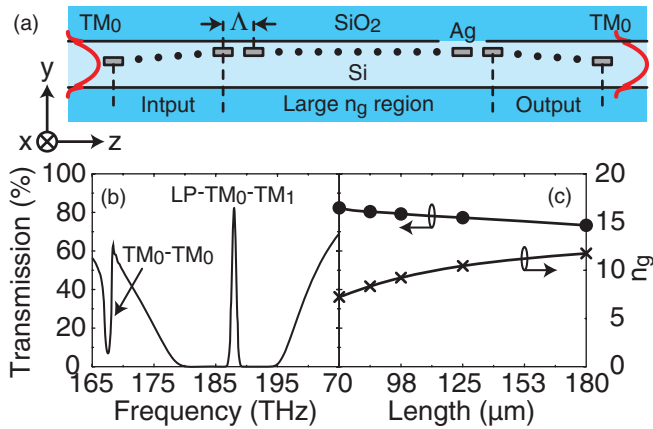
FIG. 4. (Color online) (a) A slow-light waveguide made of a large group-index region sandwiched between coupling regions. The large group-index region has 0–400 resonators located 123 nm above the core’s center, while the coupling regions have 125 resonators each with the y position gradually changed from 70 to 123 nm for adiabatic coupling. (b) Transmission spectra through the waveguide with a length of 70.75 \mu\text{m} . (c) Waveguide length dependence of transmission and averaged group index of the system.
