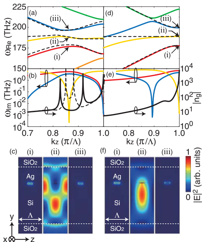
FIG. 3. (Color online) (a) Numerically calculated dispersion relations for coupled LP- TM_0 - TM_1 modes with resonators located 123 nm above the waveguide core's center. Numerical dispersion agrees with analytical one from Eq. (1) (dashed curves) using \hbar[C_0, C_1] = [28, 37] meV, \delta/2\pi = -100 GHz, and 2\gamma/2\pi = 10.5 THz. (b) Damping rates of the middle three modes (red, yellow and blue curves) and the retrieved group index of the central mode (black curve). Dashed curve is the group index when Eq. (2) is satisfied (resonator position at 130 nm above the core's center). (c) |E|^2 distributions of the middle three modes at k_z\Lambda/\pi = 0.86 , labeled as (i), (ii), and (iii) in (a). (d), (e), and (f) show the LP- TM_0 - TM_0 case with resonators located 130 nm above the core's center. The analytical dispersion (dashed curves) uses \hbar C_0 = 35 meV, \delta/2\pi = -100 GHz, and 2\gamma/2\pi = 10.5 THz. (f) |E|^2 distributions of the lower three modes at the band edge, labeled as (i), (ii), and (iii) in (d). Note that |E|^2 distributions of mode (ii) in (c) and (f) have been multiplied by 100 and 25, respectively, for clarity.
