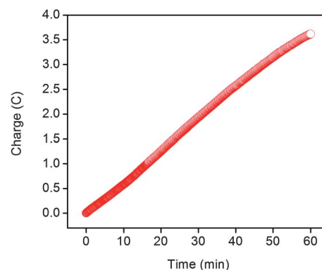
Fig. 7 Charge build-up versus time for 0.1 mM \mathbf{1}(\text{CF}_3\text{SO}_3)_2 in a 0.1 M (\text{Bu}_4\text{N})\text{PF}_6 acetonitrile solution and 17 mM of acetic acid at a glassy carbon rod electrode operating at a potential of -1.6 V vs. SHE for 1 h. Background activity of direct proton reduction at the electrode has been subtracted from the data.
