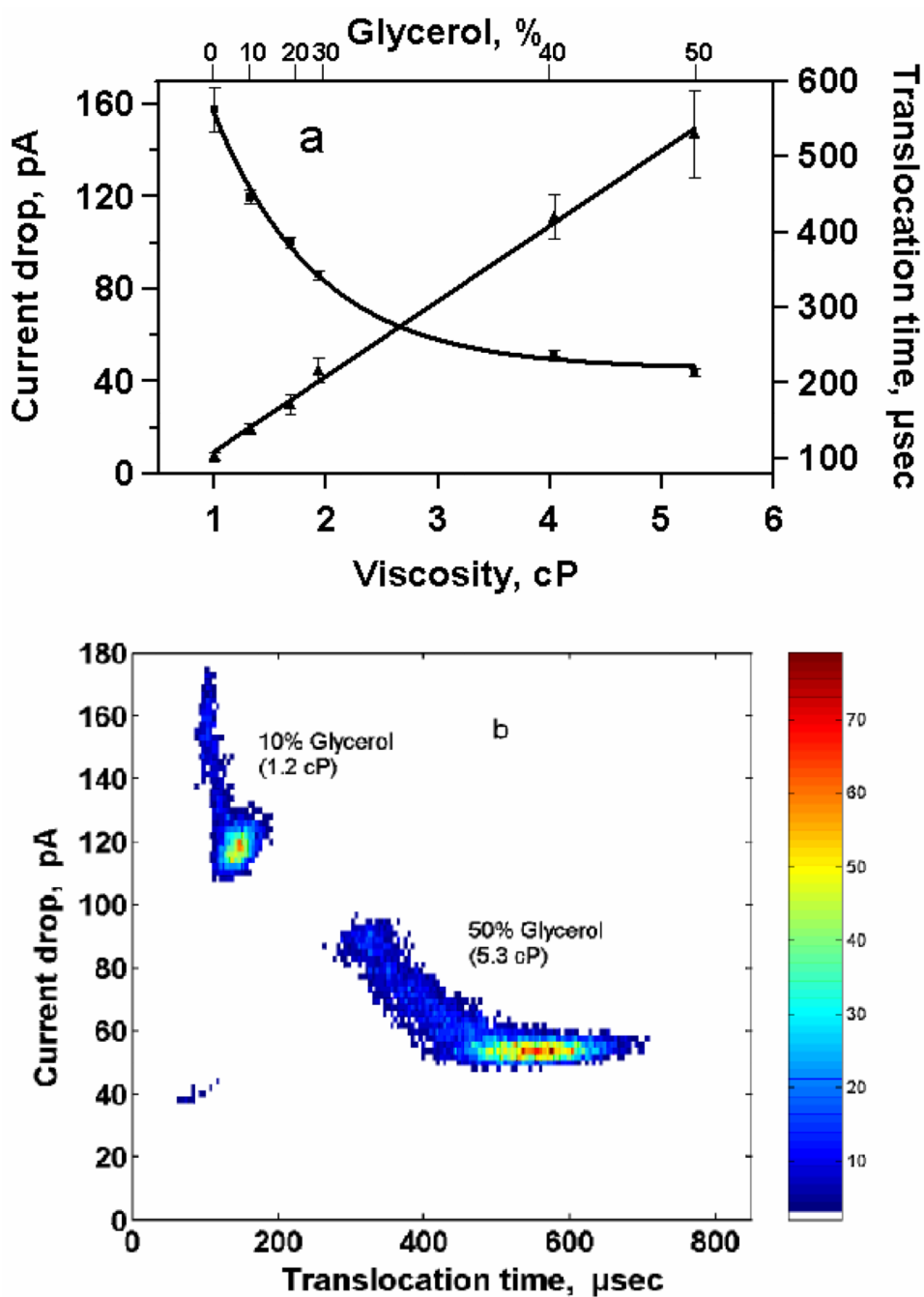
Figure 1. a) Current blockage ( \blacksquare ) and translocation time ( \blacktriangle ) versus viscosity for 3kbp DNA in 1.5 M KCl-TE solution at 120 mV bias voltage; the solid curves are fits for \Delta I_b \sim 1/\eta and t_d \sim \eta . b) The scatter plots for the addition of 10% and 50% glycerol to the ionic solution, the color scale represents the events density.
