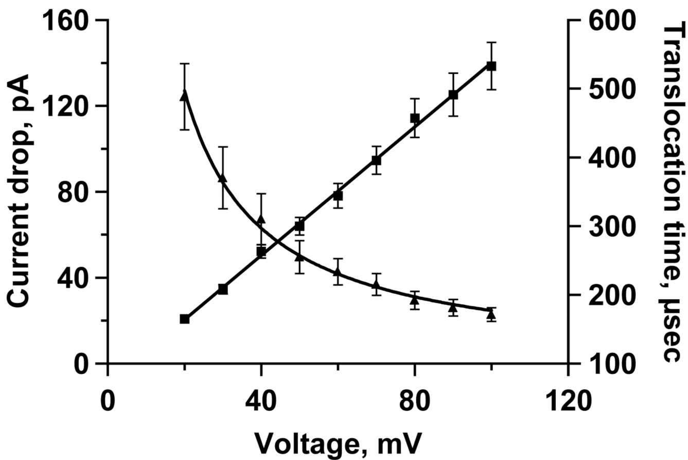
Figure 2. Current blockage (■) and translocation time (▲) versus applied voltage measured in 1.6 M KCl-TE buffer containing 20% glycerol. The solid curves represents fits where \Delta I_b \sim V and t_d \sim 1/V .
