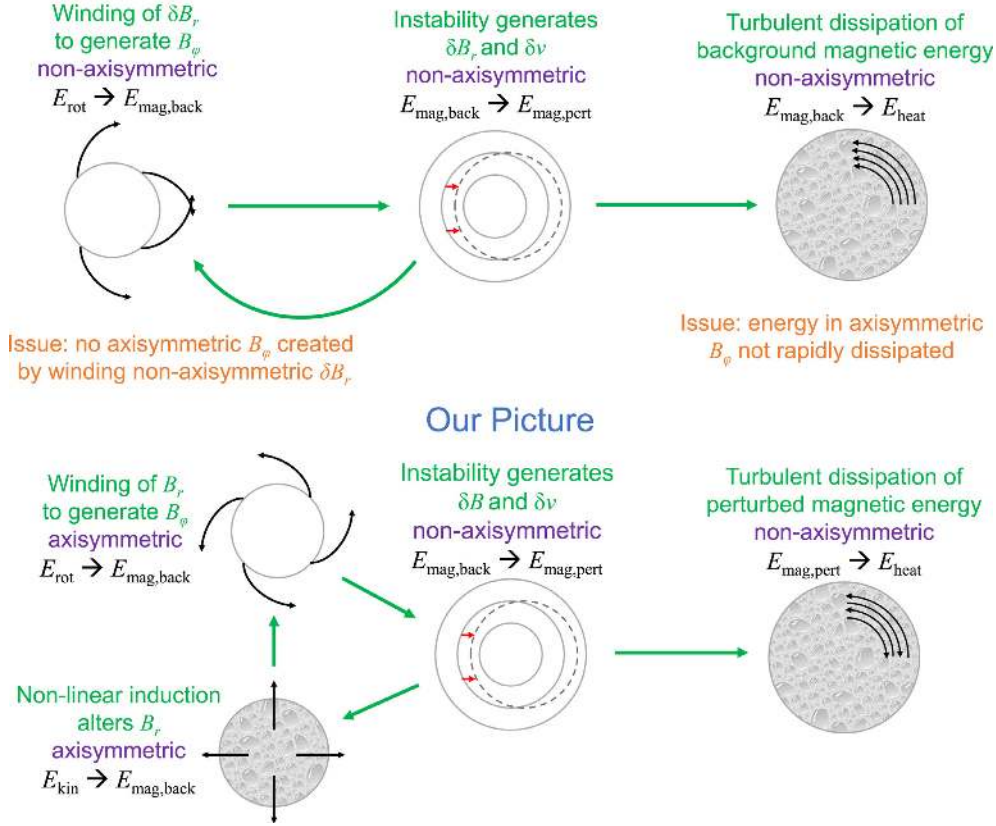
Figure 1. Schematic showing the physical processes at work in stars undergoing Taylor instability, according to the Taylor–Spruit dynamo as proposed by Spruit 2002 (top) and our model (bottom). Black arrows represent magnetic field lines, while red arrows represent fluid motions. Orange text describes processes that we argue operate differently than proposed by Spruit 2002.
