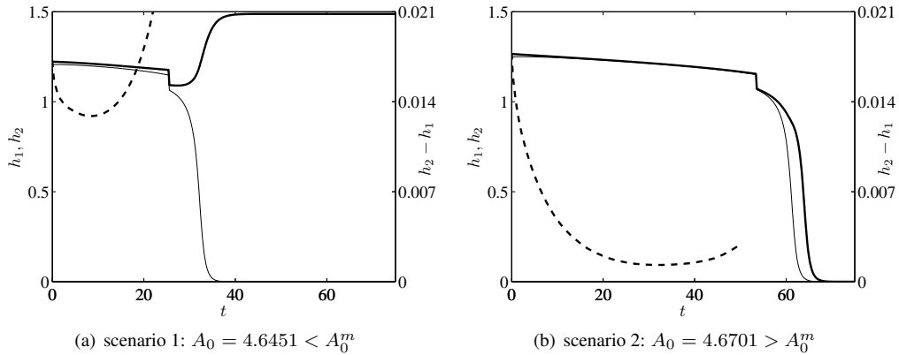
Figure 19: Plots of the amplitude of the left (light solid) and right (heavy solid) spikes versus time as A is decreased from A_0 to A_m - 0.004 . For D = 0.4 , we find from Figure 15(b) that A_- = 4.6351 , A_m = 4.6206 , and A_0^m = 4.6534 . The near-vertical kinks at t \approx 25.4 in the left figure and t \approx 53.4 in the right are the result of the addition of an even perturbation when A reaches A_m - 0.004 . The dashed curve, plotted against the right vertical axis, is a plot of the difference in spike amplitudes. In the left figure where A_0 < A_0^m , the competition mode sets in early and dominates the dynamics near the saddle. As a result, only one spike collapses. In the right figure, the competition mode has not set in by the time the even perturbation is added. The resulting dynamics are near that of a simultaneous collapse of both spikes. The presence of the competition mode causes the right spike to collapse slightly more slowly than the left.
