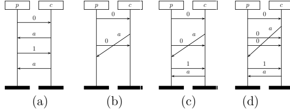
Fig. 4. The initial input scenarios for Smyle
