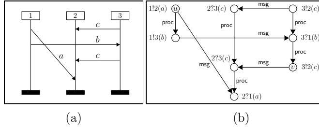
Fig. 1. An MSC (a) and its graph (b)
