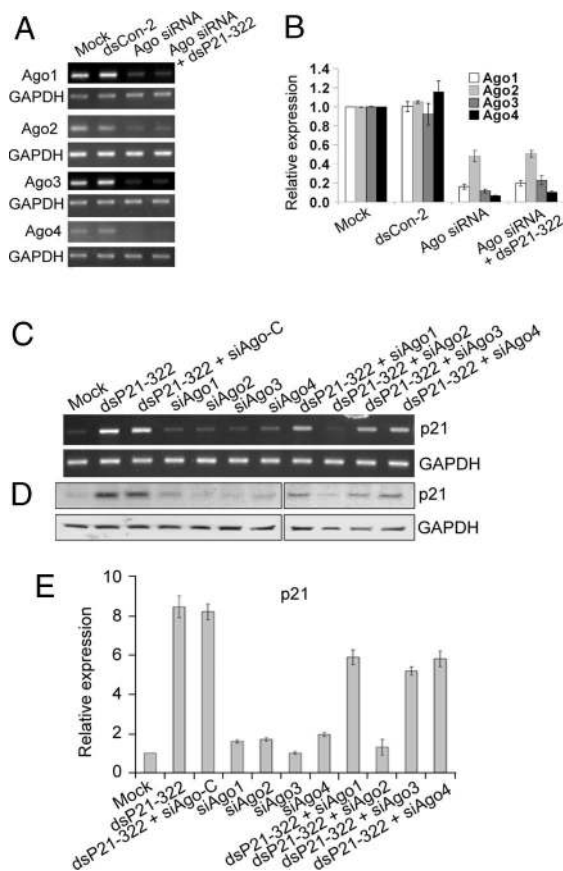
Fig. 5. RNAi requires the Ago2 protein. (A) PC-3 cells were transfected with 50 nM of the indicated dsRNA molecules for 72 h. mRNA expression of Ago1–4 was assessed by RT-PCR. Each Ago family member was knocked down by its corresponding Ago siRNA (siAgo1, 2, 3, or 4). (B) RT-PCR results were normalized to GAPDH expression levels and are presented as the mean \pm SEM from two independent experiments. (C and D) PC-3 cells were transfected with 50 nM of each indicated dsRNA for 72 h. Both p21 and GAPDH mRNA (C) and protein (D) levels were determined by RT-PCR and Western blot analysis, respectively. (E) p21 mRNA levels were normalized to GAPDH and are presented as the mean \pm SEM from at least two independent experiments (containing two sample repeats per experiment).
