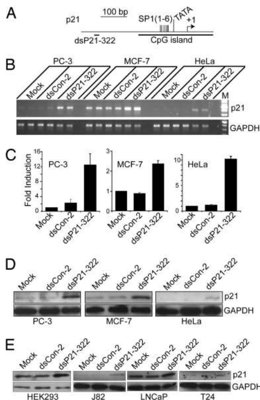
Fig. 2. dsRNAs induce p21 expression in different human cell lines. Cells were transfected with 50 nM dsRNA for 72 h. mRNA and protein levels were analyzed by RT-PCR and Western blotting, respectively. (A) A schematic representation of the p21 promoter with its CpG island, SP1 sites, TATA signal, transcription start site, and the dsRNA target. (B) p21 and GAPDH mRNA expression levels in PC-3, MCF-7, and HeLa cells after mock, dsCon-2, or dsP21-322 transfections. (C) p21 mRNA expression levels were normalized to GAPDH. The results are presented as the mean \pm SEM of two independent experiments (two sample repeats within each experiment). (D) Induction of p21 protein expression was confirmed by Western blot analysis in PC-3, MCF-7, and HeLa cells. GAPDH levels were also detected and served as a loading control. (E) Western blot analysis of p21 and GAPDH after mock, dsCon-2, or dsP21-322 transfections in HEK293, J82, LNCaP, and T24 cells.
