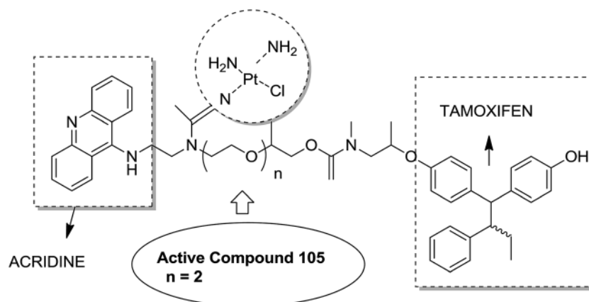
Fig. 66 Platinum-acridine-endoxifen hybrid.
