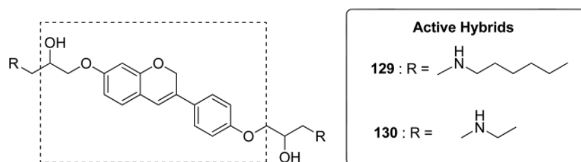
Fig. 82 Isoflavene-propranolol hybrids.
