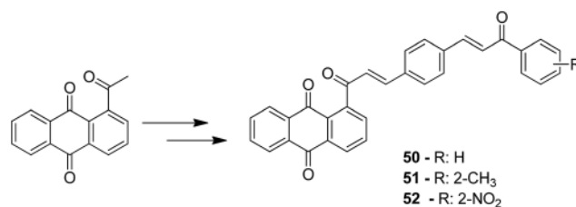
Fig. 30 Anthraquinone-chalcone hybrids.
