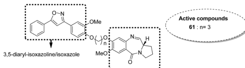
Fig. 37 3,5-Diaryl-isoxazoline/isoxazole–pyrrolobenzodiazepine conjugates.
