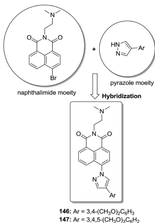
Fig. 93 Pyrazol–naphthalimide derivatives.
