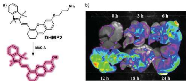
Fig. 25 (a) Chemical structure of small molecule-based NIR probe DHMP2 and working model for the chemical changes that make it useful in the detection of MAO-A activity. (b) Fluorescence images of MAO-A in liver fibrotic tissue of \text{CCl}_4 -induced fibrotic rats treated with probe DHMP2 ( 50 \mu\text{M} , 1 \text{ mL} ) at different times (0, 3, 6, 12, 18 and 24 h). \lambda_{\text{ex}} = 630 \text{ nm} , \lambda_{\text{em}} = 700 \text{ nm} . Reproduced with permission from ref. 36. Copyright (2020) American Chemical Society.
