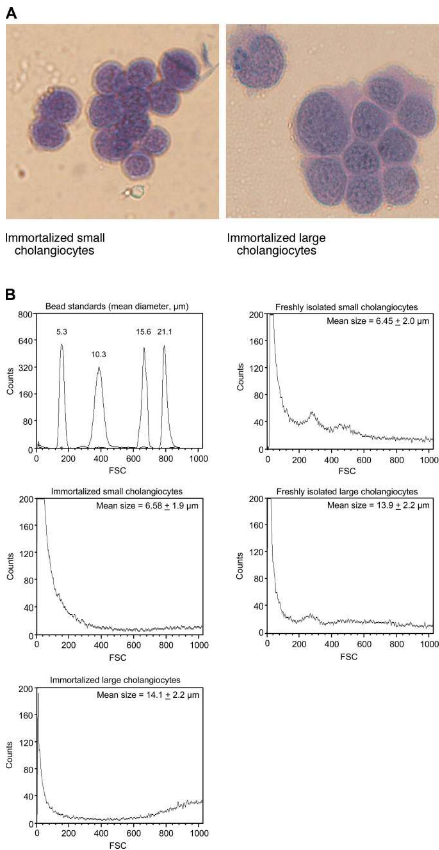
Fig. 1. A : light micrographs of immortalized small and large murine cholangiocytes. These two cell subtypes differ in morphological appearance and diameter. Original magnification \times 400 . B : size profiles of small and large cholangiocytes. Forward scatter (FSC) profiles were performed on immortalized and freshly isolated small and large cholangiocytes. The average cell diameter in each population was determined by comparing mean FSC signal with those of unstained microsphere size standards. FSC profiles of the microsphere standards are shown in top left . The average diameter (in \mu\text{m} ) provided by the manufacturer is given above each peak. Cell sizes were calculated using a regression line constructed from mean FSC profiles of the standards. Means \pm SE of FSC signals shown in histograms were determined using BD CellQuest Pro software, in which 40,000 events were recorded for each sample. C : representative immunofluorescent micrographs of immortalized small and large cholangiocytes stained for secretin receptor (SR), cystic fibrosis transmembrane conductance regulator (CFTR), \text{Cl}^-/\text{HCO}_3^- anion exchanger 2 ( \text{Cl}^-/\text{HCO}_3^- AE2), and cytokeratin-7 (CK-7). Corresponding negative controls are included. Bar = 50 \mu\text{m} .
