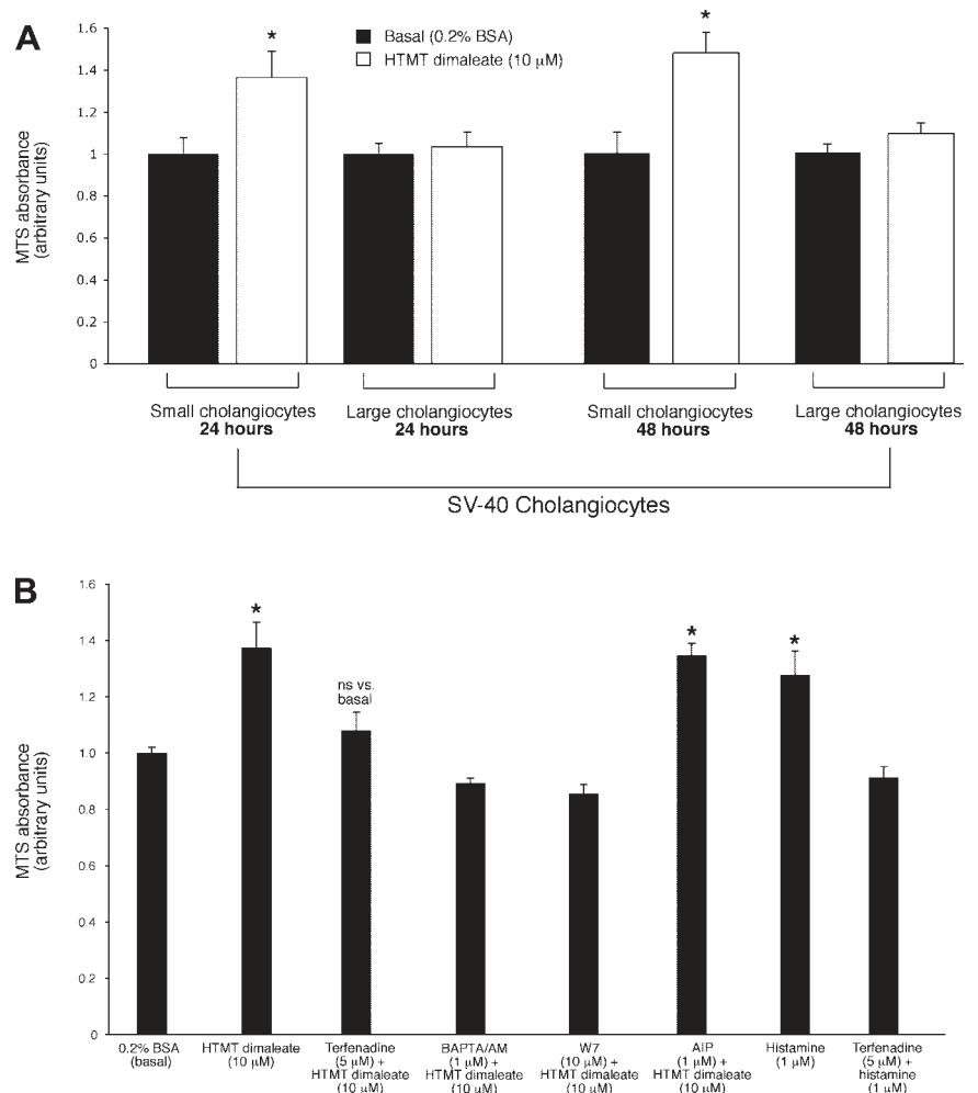
Fig. 3. A: effect of histamine trifluoromethyl toluidide (HTMT dimaleate) (10 \mu\text{M} for 24 and 48 h) on the proliferation of immortalized small and large cholangiocytes. Data are means \pm SE of 10 experiments. * P < 0.05 vs. its corresponding basal value. B: effect of HTMT dimaleate (10 \mu\text{M} for 48 h) in the absence or presence of terfenadine (5 \mu\text{M} ), BAPTA/AM (1 \mu\text{M} ), W7 (10 \mu\text{M} ), and AIP (1 \mu\text{M} ) or 2) histamine (1 \mu\text{M} for 48 h) in the absence or presence of terfenadine (5 \mu\text{M} ). Data are means \pm SE of 8 experiments. * P < 0.05 vs. its corresponding basal value.
