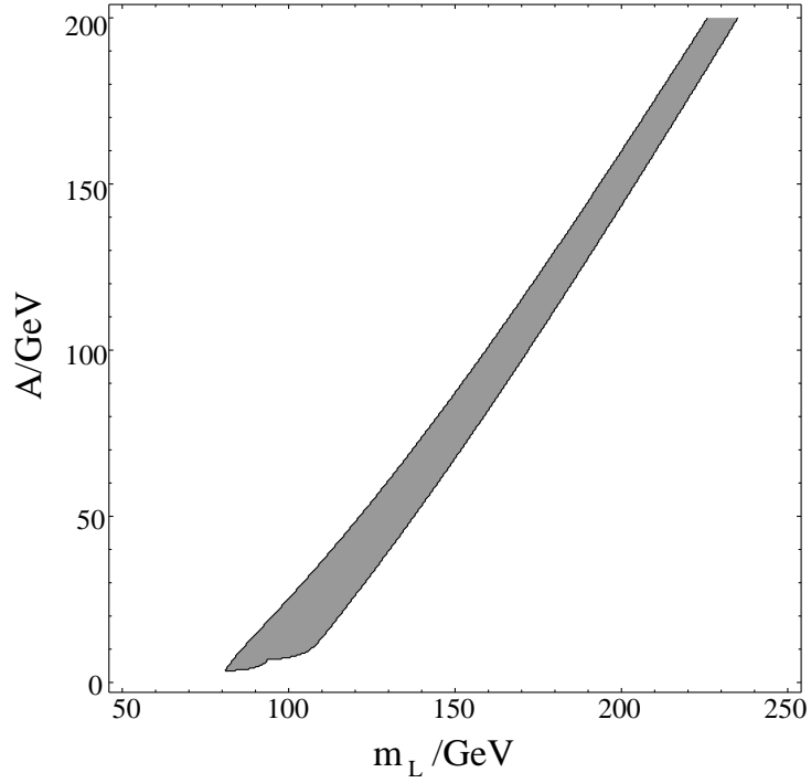
Figure 5: The region of parameter space in which the Z width constraint is met and \Gamma(h \rightarrow \tilde{\nu}\tilde{\nu}) > \Gamma(h \rightarrow b\bar{b}) holds, for \tan\beta = 2 and m_h = 130 GeV. We take the splitting between m_L and m_R to be generated by RG running from the GUT scale, as discussed in the text.
