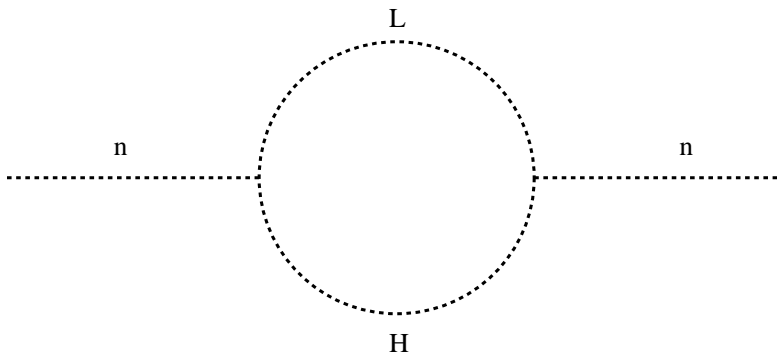
Figure 2: Loops contributing to the running of m_{\tilde{n}} .
