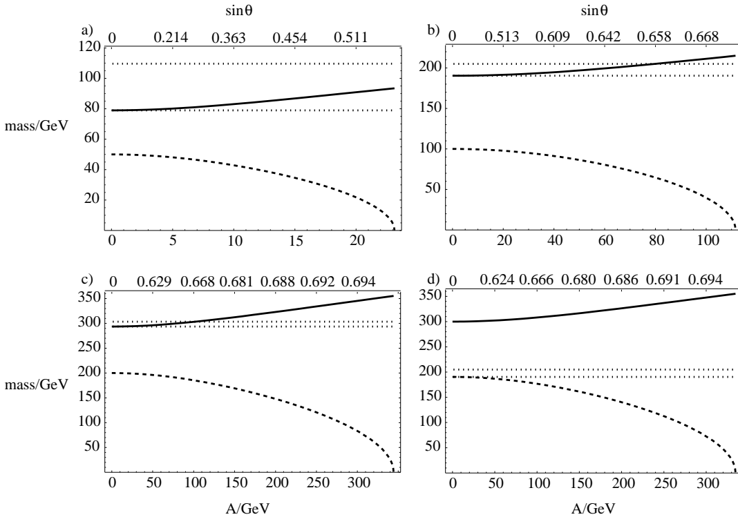
Figure 1: Slepton mass spectra as a function of A for (a) m_L = 100\text{GeV} , m_R = 50\text{GeV} , (b) m_L = 200\text{GeV} , m_R = 100\text{GeV} , (c) m_L = 300\text{GeV} , m_R = 200\text{GeV} , and (d) m_L = 200\text{GeV} , m_R = 300\text{GeV} . The solid line is the mass of the heavier sneutrino, the dashed line that of the lighter sneutrino. The dotted lines are the masses of the sneutrino (lower dotted) and charged slepton (higher dotted) in the MSSM. Curves are drawn for \tan\beta = 5 , and are relatively insensitive to \tan\beta .
