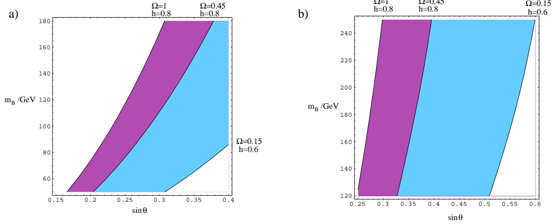
Figure 3: Contours of \Omega h^2 , where h is the normalized Hubble parameter, as a function of the bino mass m_B (assuming GUT unification of gaugino masses) and \sin \theta . Both shaded regions yield relic densities below overclosure, with the lighter shaded region corresponding to values of \Omega preferred by supernovae data [18]. In a) we take m_{\tilde{\nu}} = 10 GeV, and in b) we take m_{\tilde{\nu}} = 100 GeV, A = 20 GeV, \tan \beta = 50 , and m_h = 115 GeV. For b), direct detection bounds are evaded only in the lepton-number-violating case.
