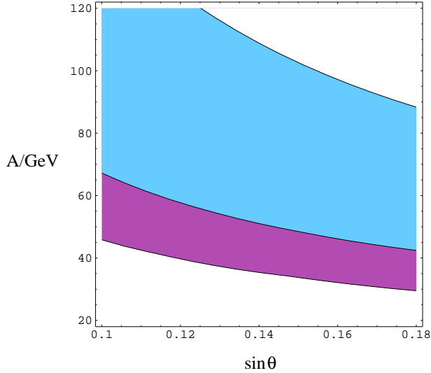
Figure 4: Contours of \Omega h^2 for m_{\tilde{\nu}} = 100 GeV as a function of \sin \theta and A . The meanings of the lighter and darker shaded regions are the same as in figures 3a) and 3b). We take \tan \beta = 50 , m_h = 115 GeV, and a bino mass of 200 GeV, and we assume GUT unification of gaugino masses.
