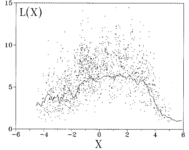
FIG. 5. The localization length, L(X) , of dipole eigenmodes vs their eigenvalues X for 500-particle CCA's. The dependence L(X) averaged over an interval of \Delta X = 0.6 for 10 random cluster realizations is shown by the solid line.
