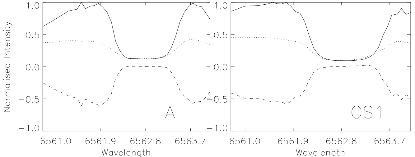
FIG. 2.— Normalised line profiles of two representative EBs compared to the background intensity of the nearby quiet Sun. The EB line profiles (solid lines) for (left) box ‘A’ and (right) box ‘CS1’ in Fig. 1 compared to the quiet Sun (dotted line). The dashed line shows the inverted (for clarity) difference in normalised intensity between the quiet Sun and EB profiles. The heightened line wings of the EB line profile are representative of other events within these data.
