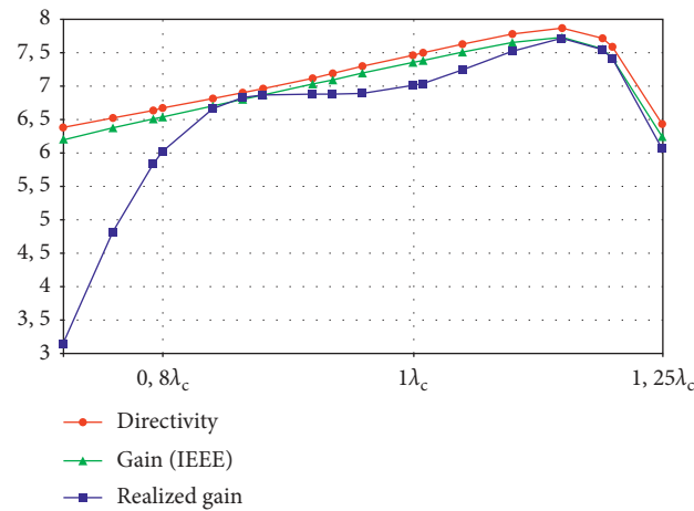
FIGURE 8: Directivity, intrinsic gain, and realized gain evolutions as a function of frequency.
