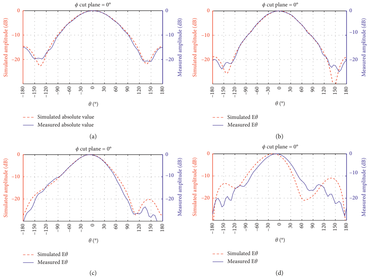
FIGURE 13: Simulation and measurement of the far-field antenna gain (E-plane) at different frequencies: (a) f=1 GHz, (b) f=1.25 GHz, (c) f=1.4 GHz, and (d) f=1.5 GHz.
