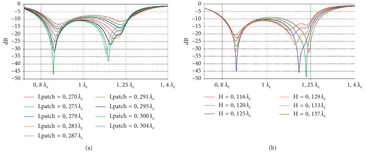
FIGURE 6: (a) S11 parameter evolution vs frequency (theoretical patch resonances when the patch is alone are positioned on the frequency axis when the patch is alone), (b) S11 parameter evolution vs frequency for the height of cavity using patch length ( L_{patch} ) excitation = 0.295\lambda_c .
