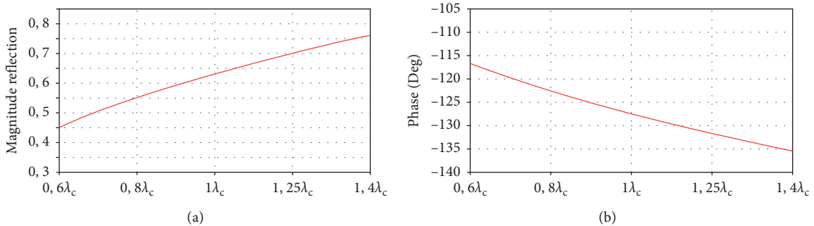
FIGURE 4: Reflection coefficient of a periodic FSS: (a) magnitude; (b) phase.
