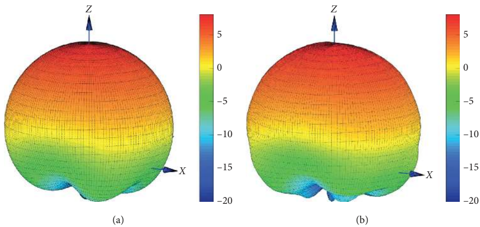
FIGURE 12: Theoretical and experimental 3D radiation patterns comparison for a central frequency at 1.25 GHz. (a) Simulation. (b) Measurement.
