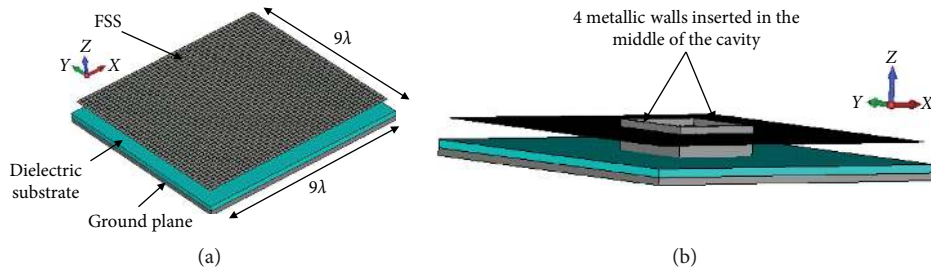
FIGURE 2: (a) High-gain EBG Antenna. (b) Vertical metallic walls inside the EBG antenna.
