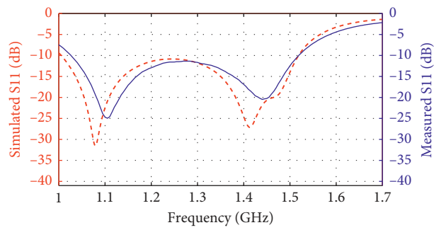
FIGURE 10: Theoretical and experimental S_{11} evolution vs frequency.
