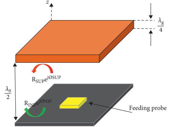
FIGURE 1: Classical EBG antenna fed by a patch.
