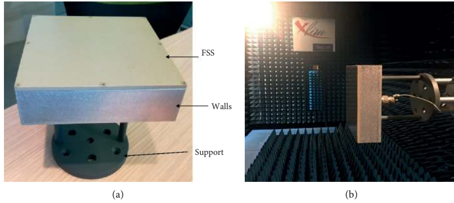
FIGURE 9: (a) Pixel antenna with supports. (b) Measurements of the radiation pattern in an anechoic chamber.
