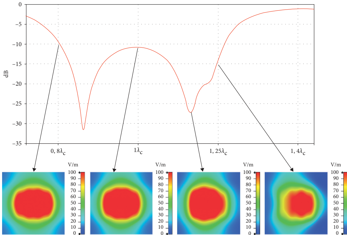
FIGURE 7: S_{11} parameter vs frequency for a 41% bandwidth and E field cartographies for some frequencies.
