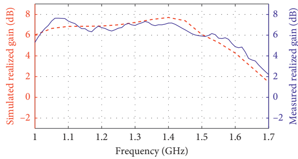
FIGURE 11: Theoretical and experimental maximum realized gains evolution vs function of the frequency.
