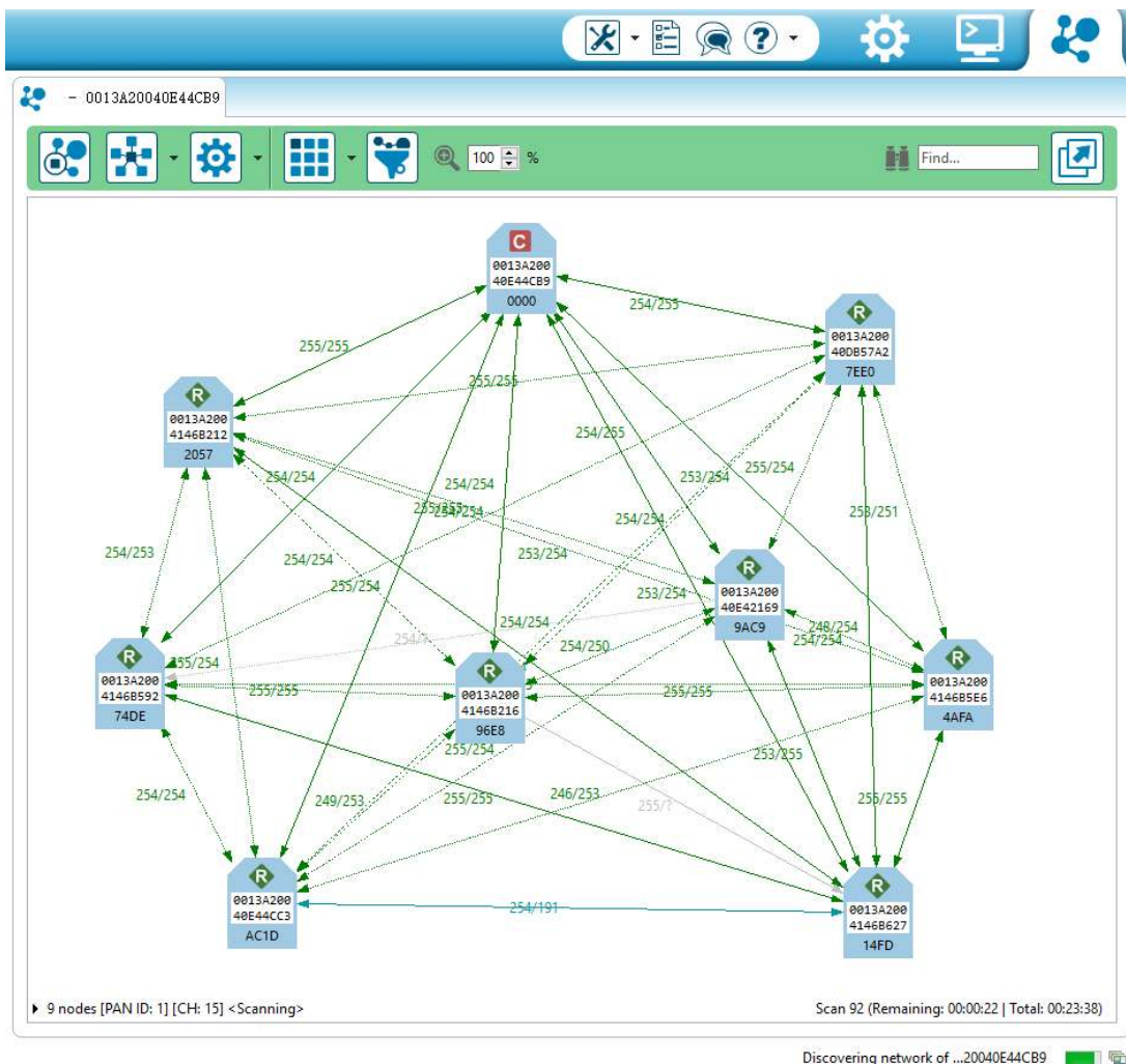
Figure 2. An XBee based WSN topology.
