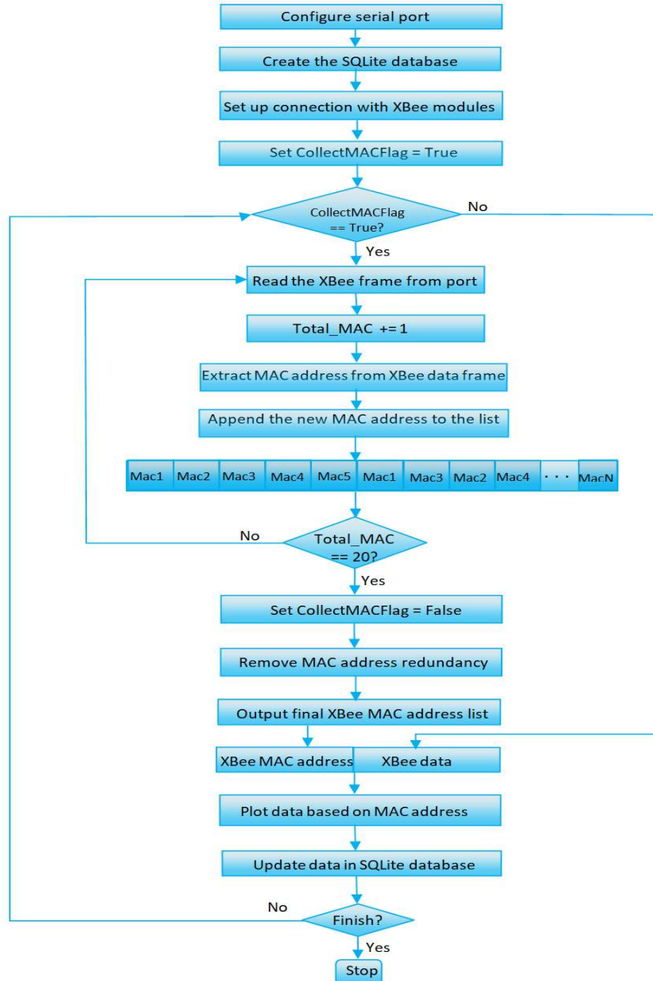
Figure 3. Algorithm flowchart of the XBee based WSN.
