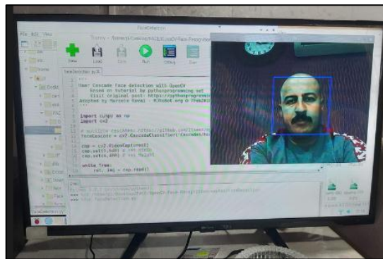
Figure 4: Face detection
