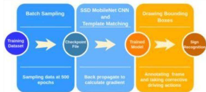
Fig. 9. Traffic Signal and Sign Detection Algorithm
