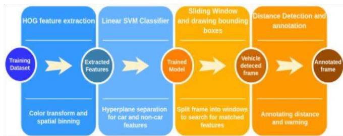
Fig. 8. Vehicle Detection Algorithm
