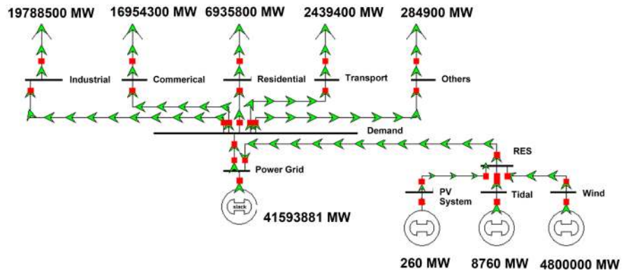
Figure 2. Illustration of overall grid connections.
