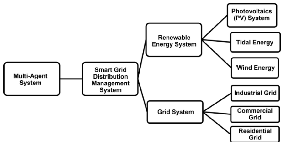
Figure 7. MAS architecture.
