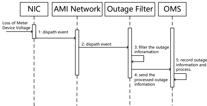
Fig. 5. Outage Notification Scenario [54]
