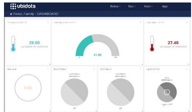
Fig. 6. Family 2 dashboard.
