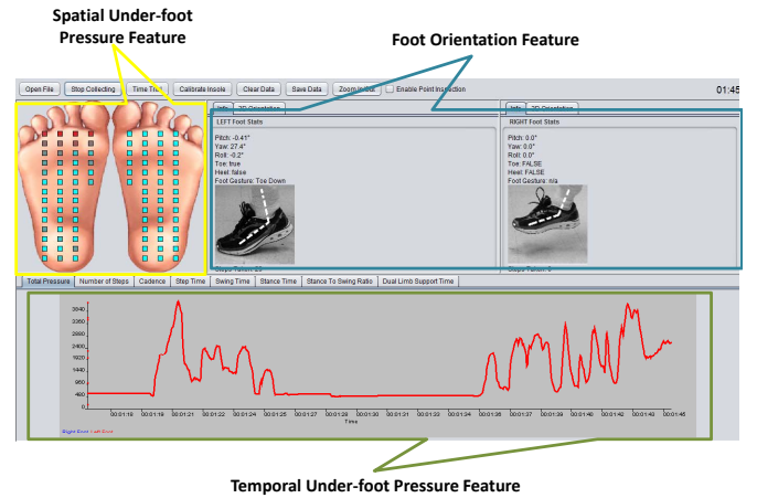
Figure 3: Software and User Interface Design
