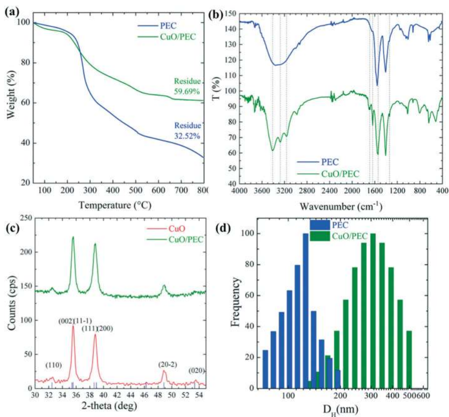
Fig. 2 (a) Thermogravimetric profiles of the PEC (blue trace) and CuO/PEC (green trace) samples. (b) Fourier-transform infrared spectra of PEC and CuO/PEC. Dashed lines refer to peaks indicative of the CuO/PEC complex formation. (c) X-ray diffraction patterns of the CuO/PEC and CuO nanopowder. The indexed peaks for the monoclinic CuO lattice are reported [JCPDS no. 41-0254]. (d) Hydrodynamic diameter, D_H , distributions for the PEC and CuO/PEC samples.
