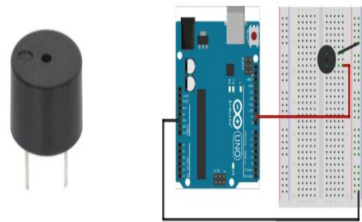
Figure 6: PIEZO buzzer
