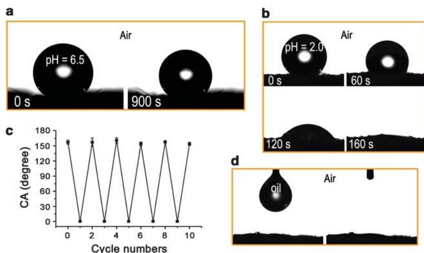
Figure 2 Wettability of the functionalized textile in air. (a) Still images from video CA measurements for a water droplet (pH=6.5) applied on the functionalized textile (left) and after 900 s of exposure (right) in air. (b) Still images from video CA measurements for a water droplet (pH=2.0) applied on the functionalized textile; the acidic droplet spread over the surface gradually within 160 s, indicating the transition of wettability of the surface from superhydrophobicity to superhydrophilicity. (c) Reversible wettability of the functionalized textile for water droplets with a pH of 6.5 (even cycles) and 2.0 (odd cycles) in air. (d) Still images from video CA measurements of a DCE droplet applied on the functionalized textile surface in air.
