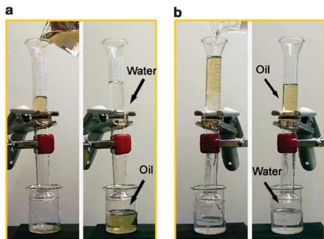
Figure 5 Controllable oil/water separation using the functionalized textile. (a) The functionalized textile was fixed between two glass tubes as the separation membrane. A mixture of gasoline and water was poured into the upper glass tube. The gasoline selectively passed through the textile, whereas the water remained in the upper glass tube (right panel). (b) The functionalized textile was first wetted with acidic water (pH=2.0) before the water/oil separation process. Water selectively passed through the textile, whereas gasoline remained in the upper glass tube (right panel).
