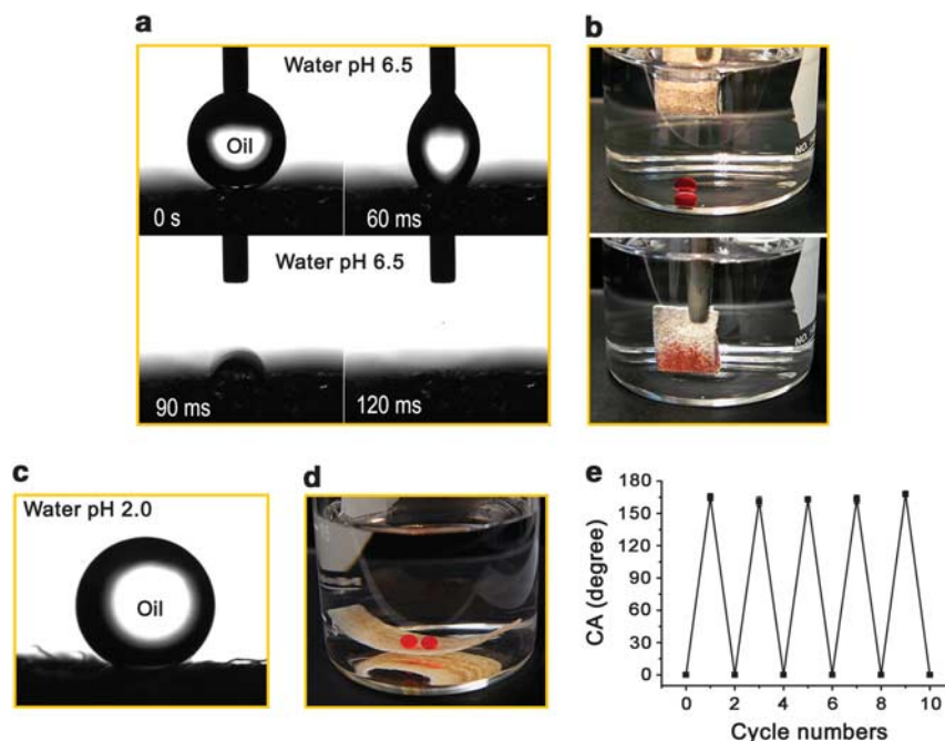
Figure 3 Oil wettability of the functionalized textile in aqueous media. (a) Still images from video CA measurements of a DCE droplet on the functionalized textile surface in water with a pH of 6.5. (b) Snapshots showing the ability of the functionalized textile for the capture of an oil droplet in aqueous media with a pH of 6.5. In greater detail, an oil droplet stained with oil red O was first dropped to the bottom of a beaker containing water with a pH of 6.5. Then, a piece of the functionalized textile was lowered into the water to approach the oil droplet. On contact, the textile immediately sucked up the oil droplet, leaving behind no oil residue. (c) Image of a DCE droplet applied on the surface of the textile in water with a pH of 2.0. (d) Photograph of DCE droplets sitting on the functionalized textile in acidic water with a pH of 2.0. The DEC droplets were stained with oil red O for clear observation. (e) Reversible oil wettability of the functionalized textile in aqueous media with a pH of 6.5 (even cycles) and 2.0 (odd cycles).
