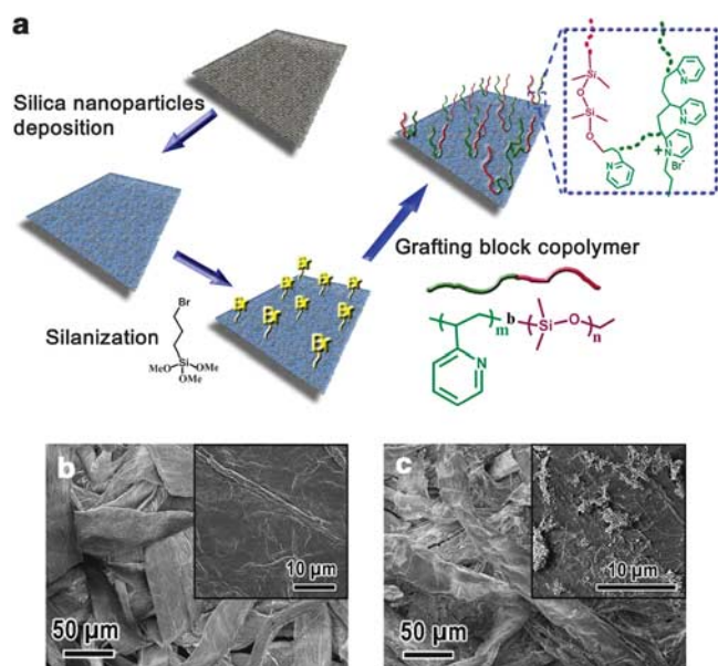
Figure 1 Preparation and characterization of a surface with switchable superoleophilicity and superoleophobicity on a non-woven textile substrate. (a) Schematic showing the preparation strategy for a surface with switchable superoleophilicity and superoleophobicity on a non-woven textile. (b) Scanning electron microscope (SEM) image of the raw textile. Inset: enlarged view of the surface of a single fiber. (c) SEM image of the textile after deposition of silica nanoparticles and block copolymer grafting. Inset: enlarged view of the surface of a single fiber.
