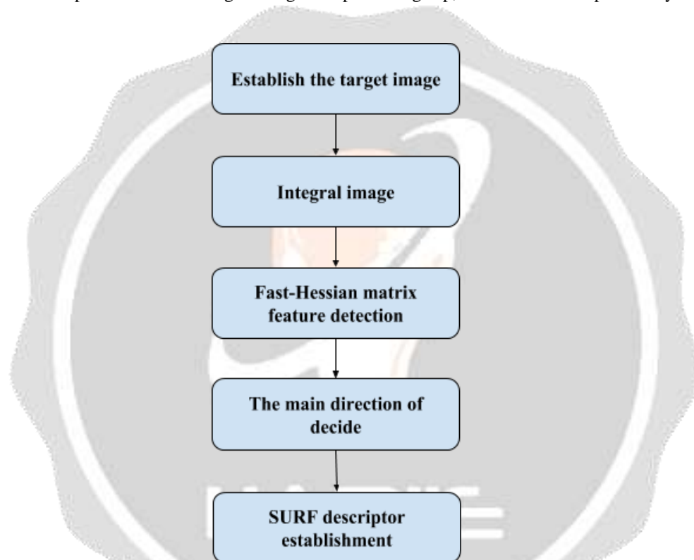
Figure 5. The training process for SURF technique
