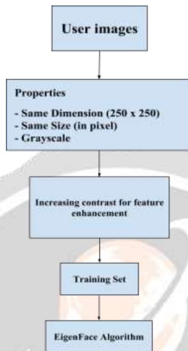
Figure 2. The training process for Eigenface technique
