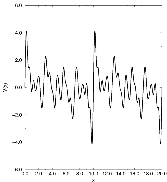
FIG. 1. Diagram of a one-dimensional random potential energy surface from a sum of Fourier sine waves with periodic boundary condition.
