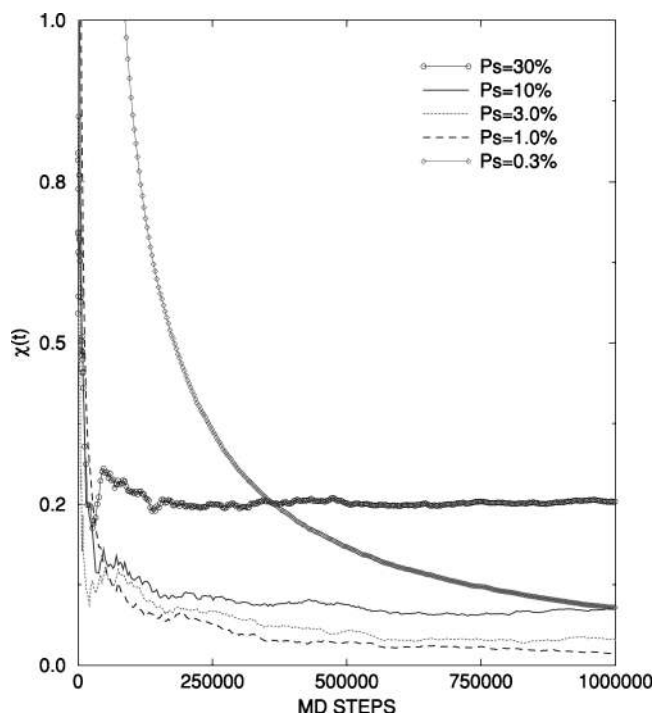
FIG. 4. The decay of \chi(t) with time, i.e., the number of MD steps in HMC, for the 1D rugged potential surface at temperature T^*=0.1 using various jumping probability P_S in S-Walking. The results show that the optimal S-Walking jump probability is about 1–10% for this 1D system.
