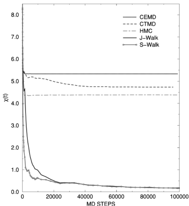
FIG. 2. A plot of \chi , as defined in Eq. (1), versus the number of MD steps for the 1D rugged potential surface at temperature T^*=0.1 using various methods. It is shown that constant energy MD (CEMD) and constant temperature MD (CTMD) methods cannot cross barriers efficiently. The hybrid Monte Carlo (HMC) method improves the ergodic sampling to some extent at this temperature. Both the J-Walking (J-Walk) and S-Walking (S-Walk) methods work very well, with S-Walking working a little better. However, as we will see later, the S-Walking method will be much more efficient than the J-Walking method in real protein systems.
