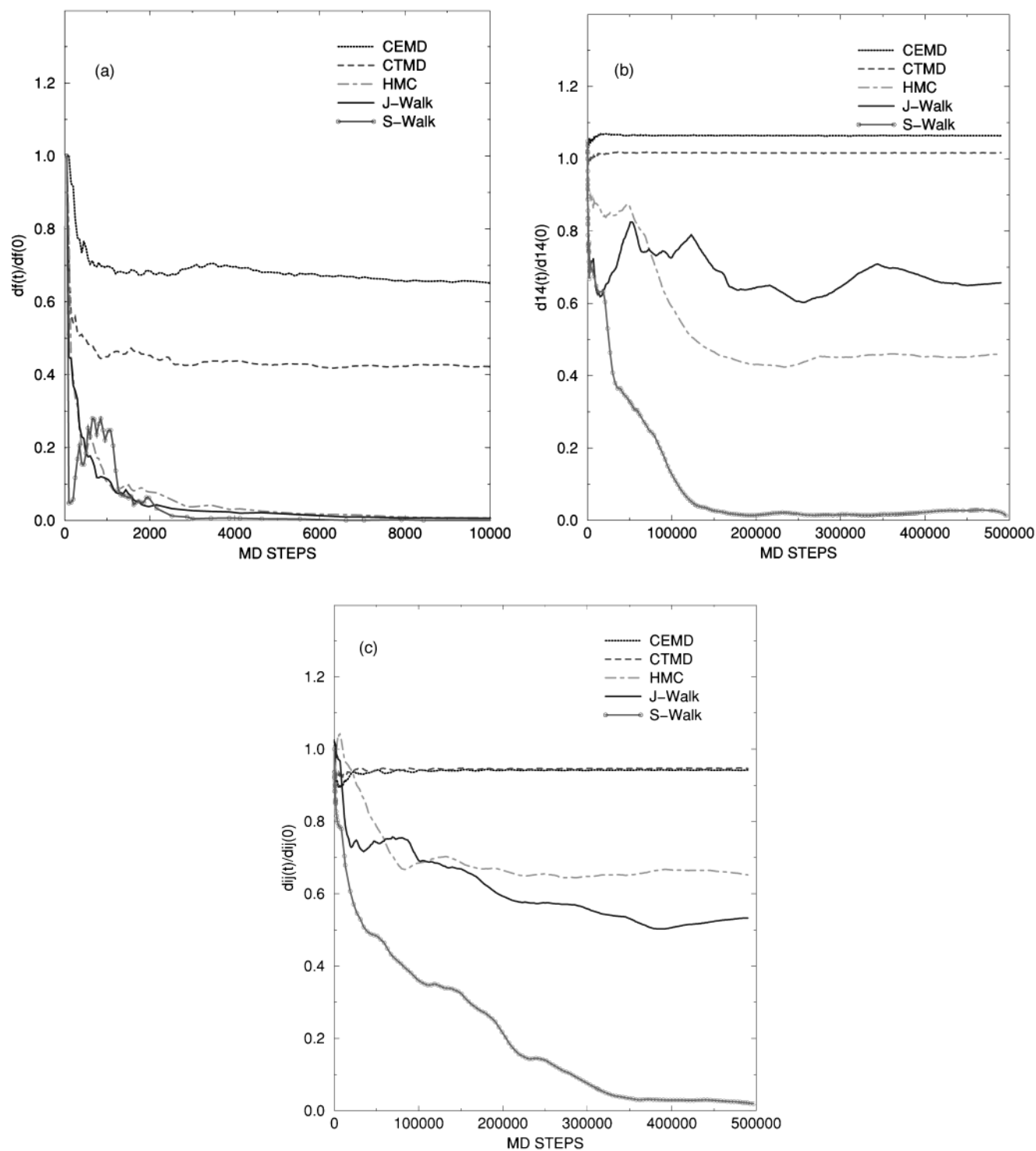
FIG. 5. Decay of the three ergodic measures with the number of MD steps for the pentapeptide Met-enkephalin using various sampling methods: (a) force magnitude metric df(t) ; (b) 1,4-pair distance metric d14(t) ; (c) all-pair distance metric dij(t) . It should be noted that the CPU time for J-Walking is about twice that of regular MD or HMC, and the CPU time for S-Walking is about three times that of regular MD or HMC. See the text for details.
