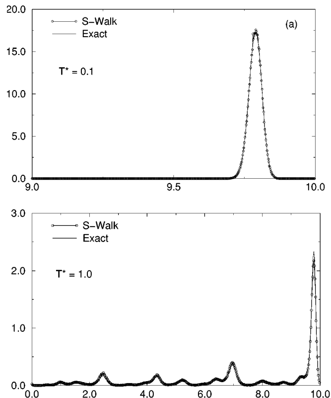
FIG. 3. A comparison of the probability distribution function, \rho(x) , obtained from S-Walking simulation and from the exact evaluation, for two different temperatures: (a) T^* = 0.1 , (b) T^* = 1.0 . The results show that the S-Walking method with P_S = 3\% generates correct Boltzmann distributions for both temperatures.
