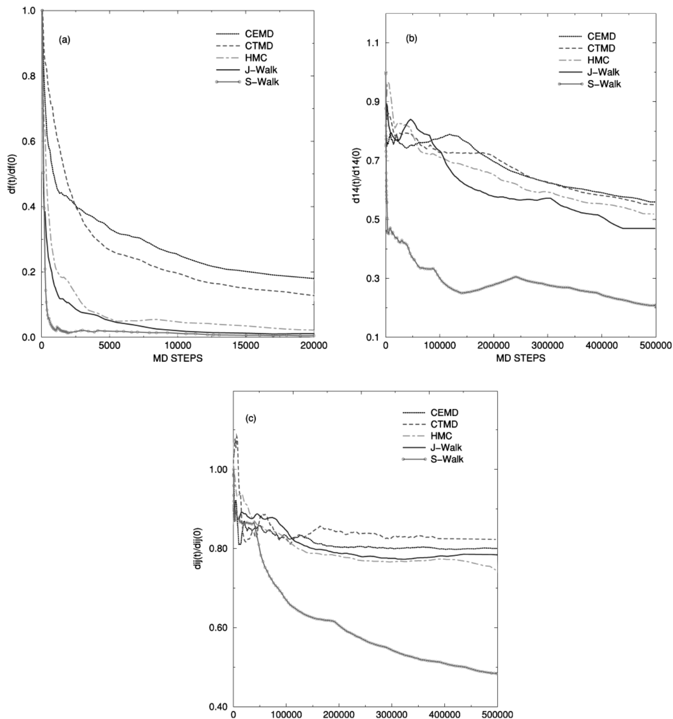
FIG. 6. Decay of the three ergodic measures with the number of MD steps for the protein melittin (PDB file 2mlt) using various sampling methods: (a) force magnitude metric df(t) ; (b) 1,4-pair distance metric d14(t) , (c) all-pair distance metric dij(t) . It should be noted that the CPU time for J-Walking is about twice that of regular MD or HMC, and the CPU time for S-Walking is about three times that of regular MD or HMC. See the text for details.
