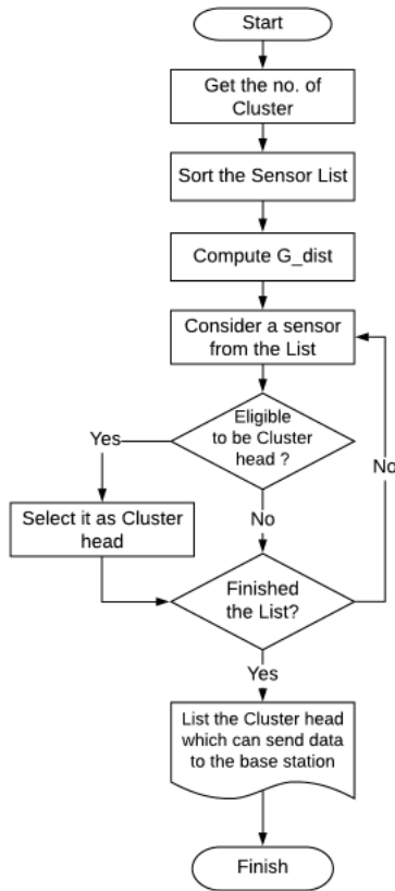
FIGURE 4. Flowchart of the proposed cluster-head selection algorithm.
