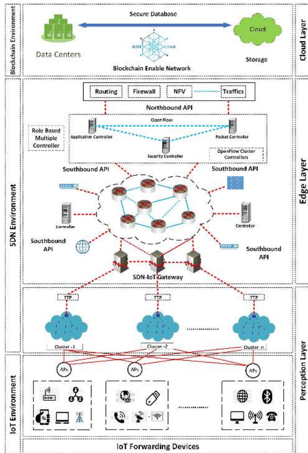
FIGURE 1. Layered architecture of Blockchain-enabled SDN-IoT ecosystem.
