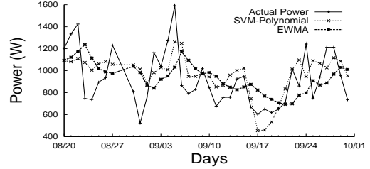
Figure 5: Predicting energy consumption using the past does not capture day-to-day variations due to changing weather, weekly routines, holidays, etc.
