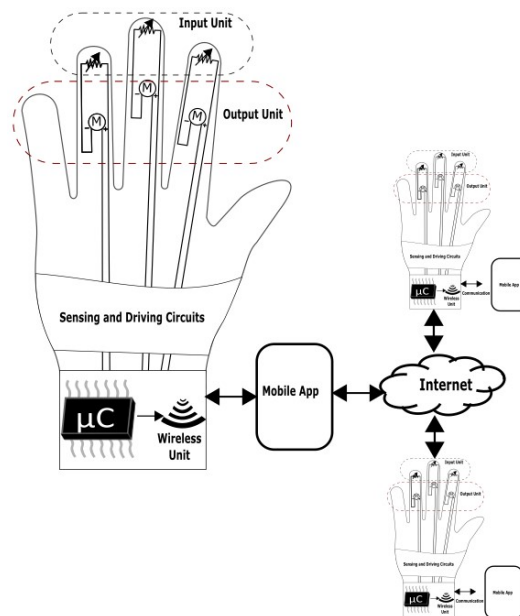
Fig. 2. Modular description of the proposed system
