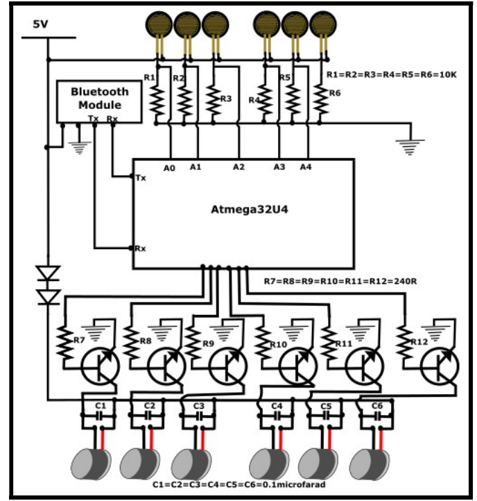
Fig.4. Simplified functional circuit diagram of the smart glove
