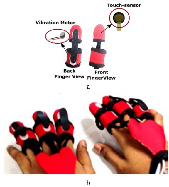
Fig.5. (a) A single-finger glove (b) SmartFingerBraille glove worn on the hand.
