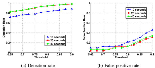
Fig. 6. Constant speed study: Performance of detecting user spoofing attack by using the same duration of run-time measurement trace and user profile trace.
