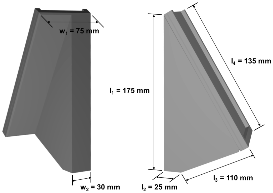
Figure S1. The mechanical dimensions of the optical cradle. The cradle is primarily divided into two distinct parts: the smartphone-holding section and the optical components section. Widths ( w_1 and w_2 ) and lengths ( l_1 , l_2 , l_3 , and l_4 ) are specified in the drawing.
