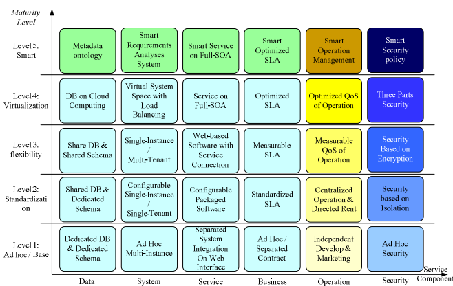
Figure 1. SmartSaaS Maturity Model.
